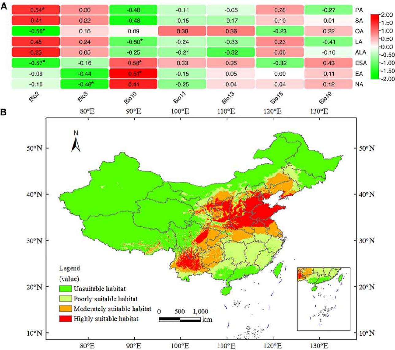
Fig. 5 The correlation analysis between bioclimatic factors and relative contents of seed FAs and potential habitats of A. truncatum . (A) The relationship between bioclimatic factors and relative contents of A. truncatum seed FAs collected from different locations. The scale bar refers to row scale. (B) Modeling environmentally suitable areas for the potential habitats of A. truncatum . The figure is based on the prediction of the maximum entropy model using MaxEnt software for species habitat modeling (v3.4.4), and the map was generated by ArcMap 10.7 (ESRI, Redlands, CA, USA, http://www.esri.com/ )
