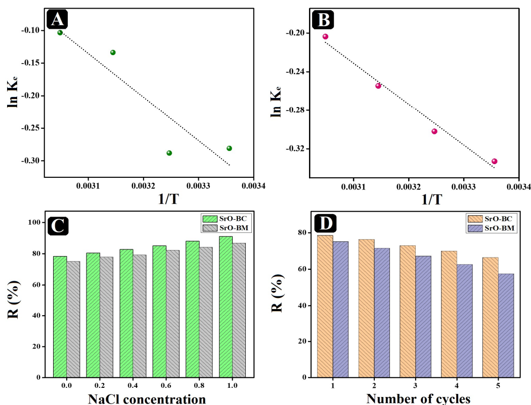
Figure 9. Van't Hoff curves of the o-NP adsorption onto (A)SrO-BC and (B)SrO-BM. (C)The impact of ionic strength on adsorbing o-NP onto SrO-BC and SrO-BM. (D)The cycling test of SrO-BC and SrO-BM during five o-NP adsorption cycles.
