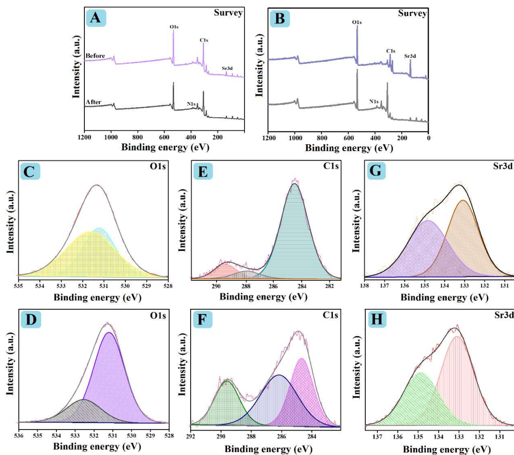
Figure 10. XPS of spectra the used SrO-BC (A) survey, (C) O1s, (E) C1s, and (G) Sr3d and the used SrO-BM (B) survey, (D) O1s, (F) C1s, and (H) Sr3d.
