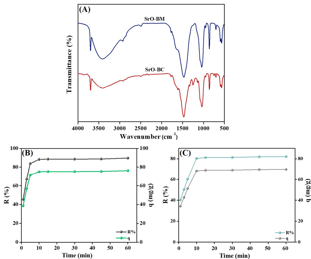
Figure 12. (A) FTIR spectra of the used SrO-BC and SrO-BM and the adsorption performance of (B) SrO-BC and (C) SrO-BM in removing o-NP from real wastewater.
