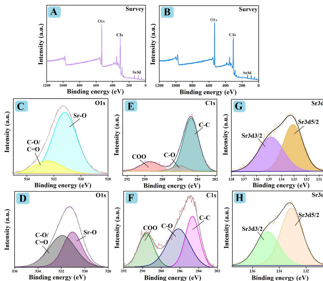
Figure 4. XPS of spectra SrO-BC (A) survey, (C) O1s, (E) C1s, and (G) Sr3d and SrO-BM (B) survey, (D) O1s, (F) C1s, and (H) Sr3d.
