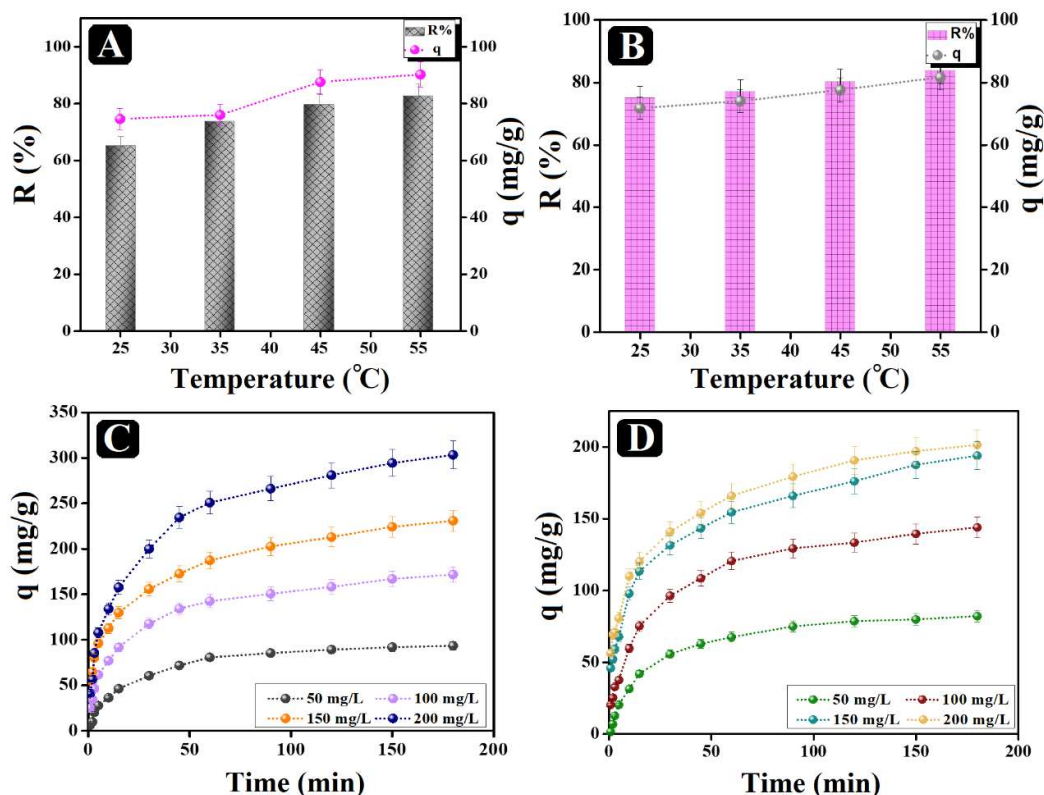
Figure 6. Effect of process temperature on adsorbing o-NP by (A) SrO-BC and (B) SrO-BM. Effect of elevating the o-NP concentrations on the o-NP adsorption aptitude onto (C) SrO-BC and (D) SrO-BM.
