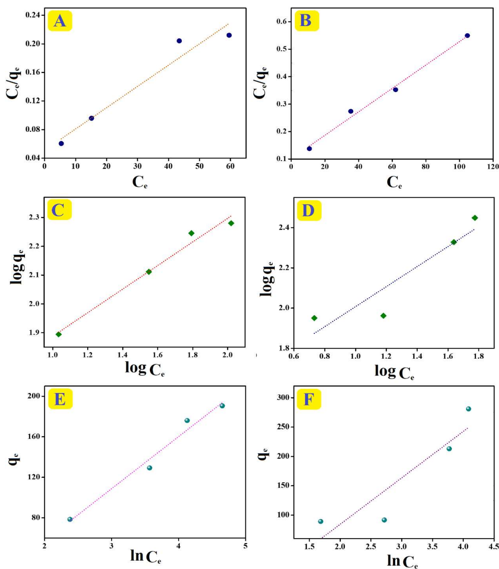
Figure 7. Langmuir, Freundlich, and Temkin curves of the o-NP adsorption processes: (A, C, E) onto SrO-BC and (B, D, F) onto SrO-BM.
