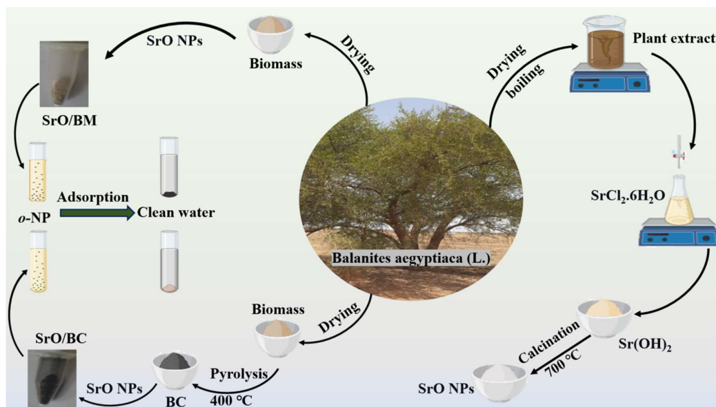
Figure 1. Eco-friendly route to fabricate Sr-BM and Sr-BC composites.
