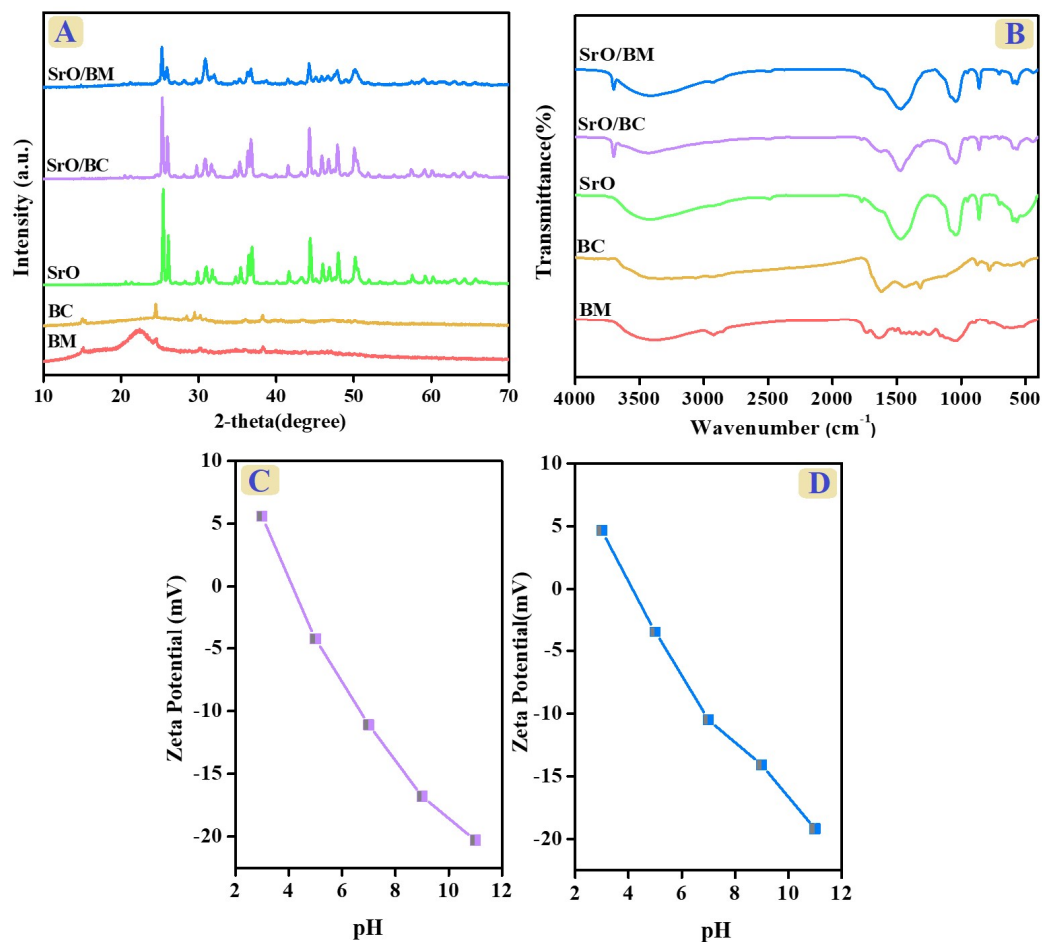
Figure 3. (A) XRD, (B) FTIR of BM, BC, SrO, SrO-BC, and SrO-BM, (C, D) ZP of SrO-BC, and SrO-BM.
