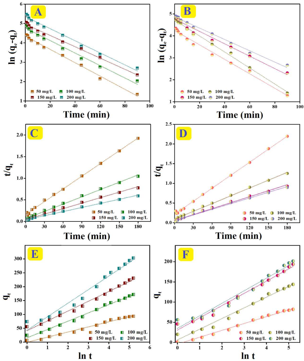
Figure 8. Pseudo-First-Order, Pseudo-Second-Order, and Elovich curves of the o-NP adsorption processes: (A, C, E) onto SrO-BC and (B, D, F) onto SrO-BM.
