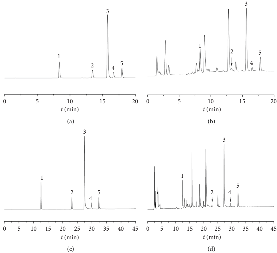
FIGURE 3: Chromatograms of the standard solutions and sample solutions. (1) Ethyl gallate. (2) Astragalín. (3) Quercetin. (4) Luteolin. (5) Kaempferol. (a) Mixed standard solution (UPLC); (b) sample solution (UPLC); (c) mixed standard solution (HPLC); (d) sample solution (HPLC).
