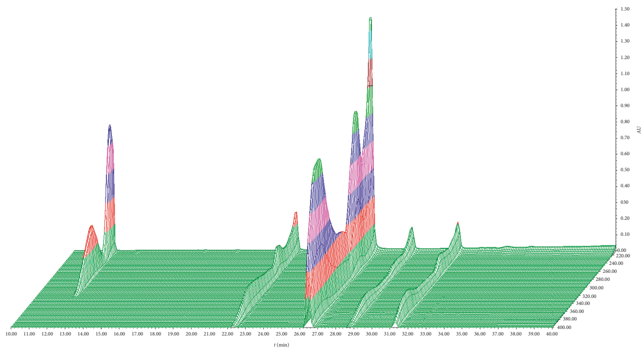
FIGURE 2: Full spectrum scan of five compounds.
