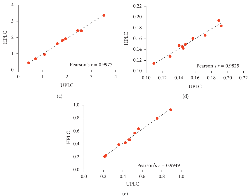
FIGURE 4: The similarity of detection results of different compounds by different chromatographic systems. (a) C 1 , (b) C 2 , (c) C 3 , (d) C 4 , and (e) C 5 .
