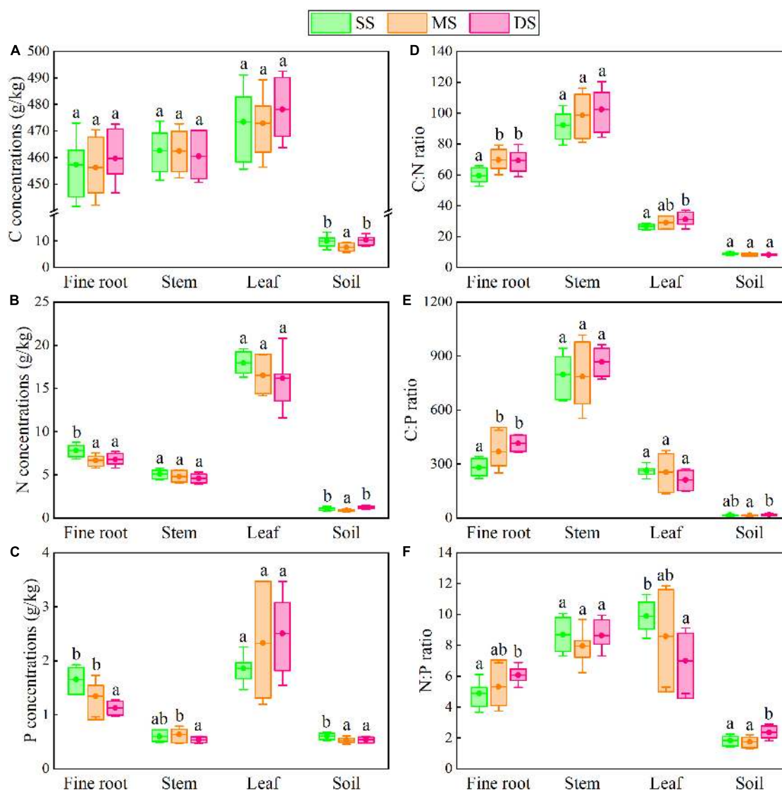
FIGURE 3 The C, N, and P concentrations (A–C) and stoichiometry (D–F) in fine roots, stems, leaves, and soils of T. distichum under different submergence treatments. Data shows a significant difference with different lowercase letters ( p < 0.05 ) in different submergence treatments (mean with standard error). The boxes give the 25 and 75% percentiles.
