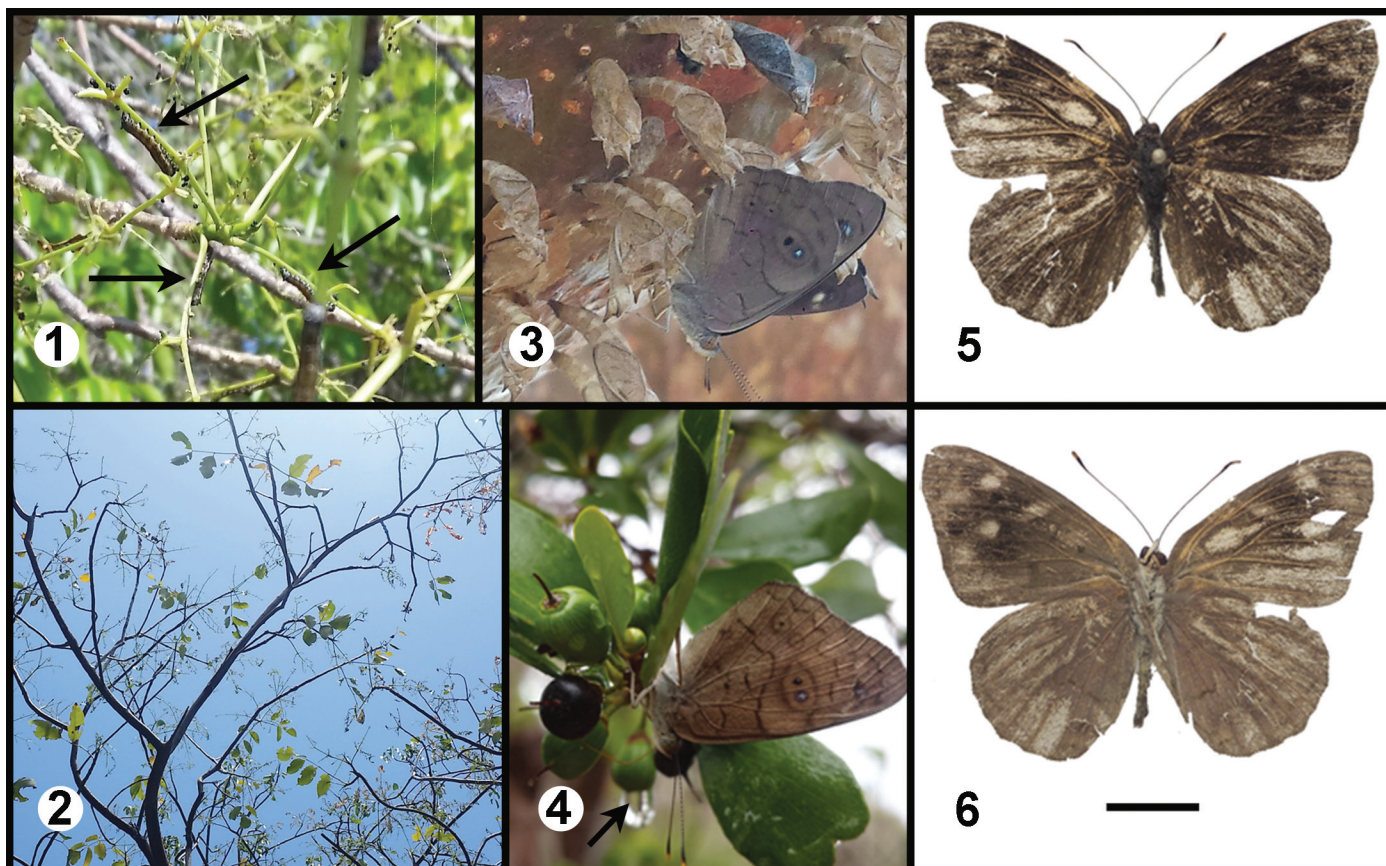
Figs. 1 and 2. Eunica monima outbreak on Bursera simaruba trees on Desecheo Island, Puerto Rico, Apr 2016, following island-wide invasive rat removal. Note that the level of damage from herbivory by larvae has left the majority of the tree canopy branches leafless (both photos). Photos by Aaron B. Shiels, 8–10 Apr 2016. Figs. 3–6. Eunica monima adults collected during their outbreak (Apr 2016) in a Bursera simaruba dominated forest on Desecheo Island, Puerto Rico, following island-wide invasive rat removal. 3. Adult and abundant empty chrysalises on the trunk of B. simaruba . 4. Adult feeding on juices from fruit of Sideroxylon obovatum Lamarck (Sapotaceae) (photos by Juan G. García-Cancel, 14–16 Apr 2016). 5 and 6. Voucher specimen (dorsal and ventral aspects) collected from Desecheo and genetically analyzed to confirm species identification (specimen was unfortunately rubbed and tattered when received). Collection data: USA, Puerto Rico, Desecheo Island, 18.385437°N, 67.480044°W, 8 Apr 2016; collector: A. B. Shiels (photos by William P. Haines).
