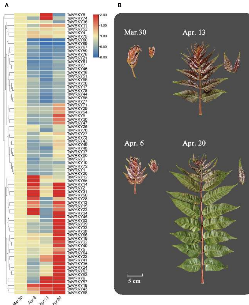
FIGURE 8 Differential transcription of TsWRKY genes in four different sampling periods (March 30, April 6, April 13, and April 20, 2021). (A) Blue and red indicate lower and higher transcript abundance, respectively, compared to initial data (March 30). (B) Samples of T. sinensis leaves from four periods.
