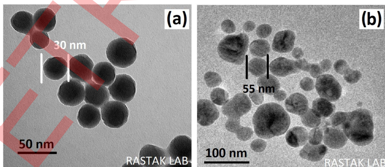
Fig 7. TEM images of (a) CS-SiO 2 NPs and (b) GS-SiO 2 NPs.
