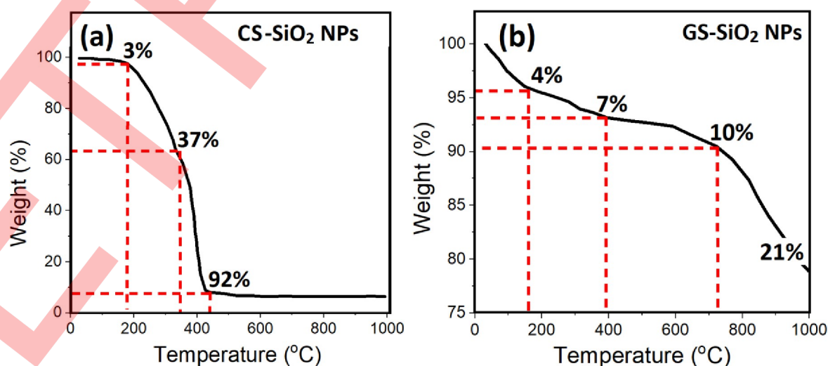
Fig 11. TGA analysis for (a) CS-SiO 2 NPs and (b) GS-SiO 2 NPs.
