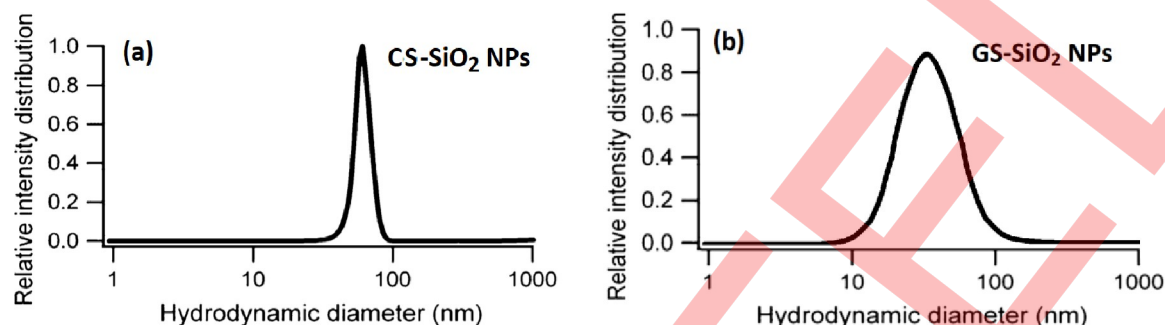
Fig 8. DLS for (a) CS-SiO 2 NPs and (b) GS-SiO 2 NPs.
