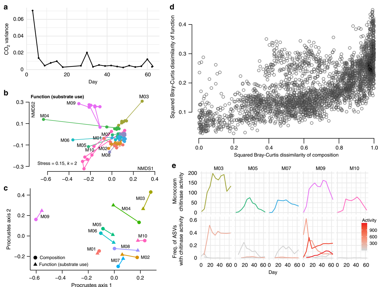
Fig. 4 Community composition strongly correlates with functional activity. a Variance in percent CO 2 among the ten microcosms over the course of the serial transfer experiment. b Two-dimensional NMDS plot of the Bray-Curtis dissimilarities of functional activity (substrate use) as measured by EcoPlates. The microcosm name is listed in black next to the Day 0 point, and the lines connect the timepoints. c Procrustes rotation of the composition NMDS plot with the function NMDS plot for Day 63 (Procrustes correlation = 0.8991, p = 0.001 ). d Plot of Bray-Curtis dissimilarities in composition between all measured timepoints across all microcosms compared with the dissimilarities in functional profile for the corresponding samples (Mantel test r = 0.6403 , p = 1 \times 10^{-4} ), squared to better illustrate the spread of points. e Endochitinase activity over time for the five microcosms that strains were cultured from (top row) and frequency of the ASVs over time that map to strains with measurable endochitinase activity (bottom row). Endochitinase activity is shown in units/mL for the strains/ASVs in the bottom row by a gradient from gray (low activity) to red (high activity).
