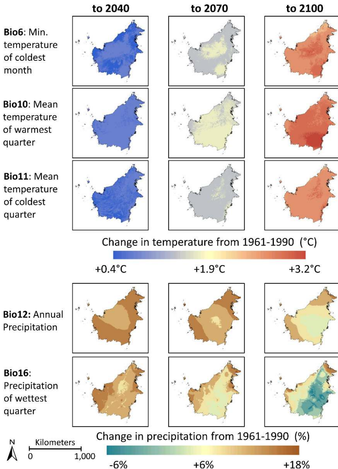
Fig 3. Projected changes in important Bioclim variables on the island of Borneo identified in Table 1. Images represent changes in Bioclim variables relative to the 1961–1990 climate surfaces, projected to 2040, 2070, and 2100. Changes in temperature variables (Bio6, Bio10, and Bio11) are presented as °C; changes for precipitation variables (Bio12, Bio16) are presented as percentages.
