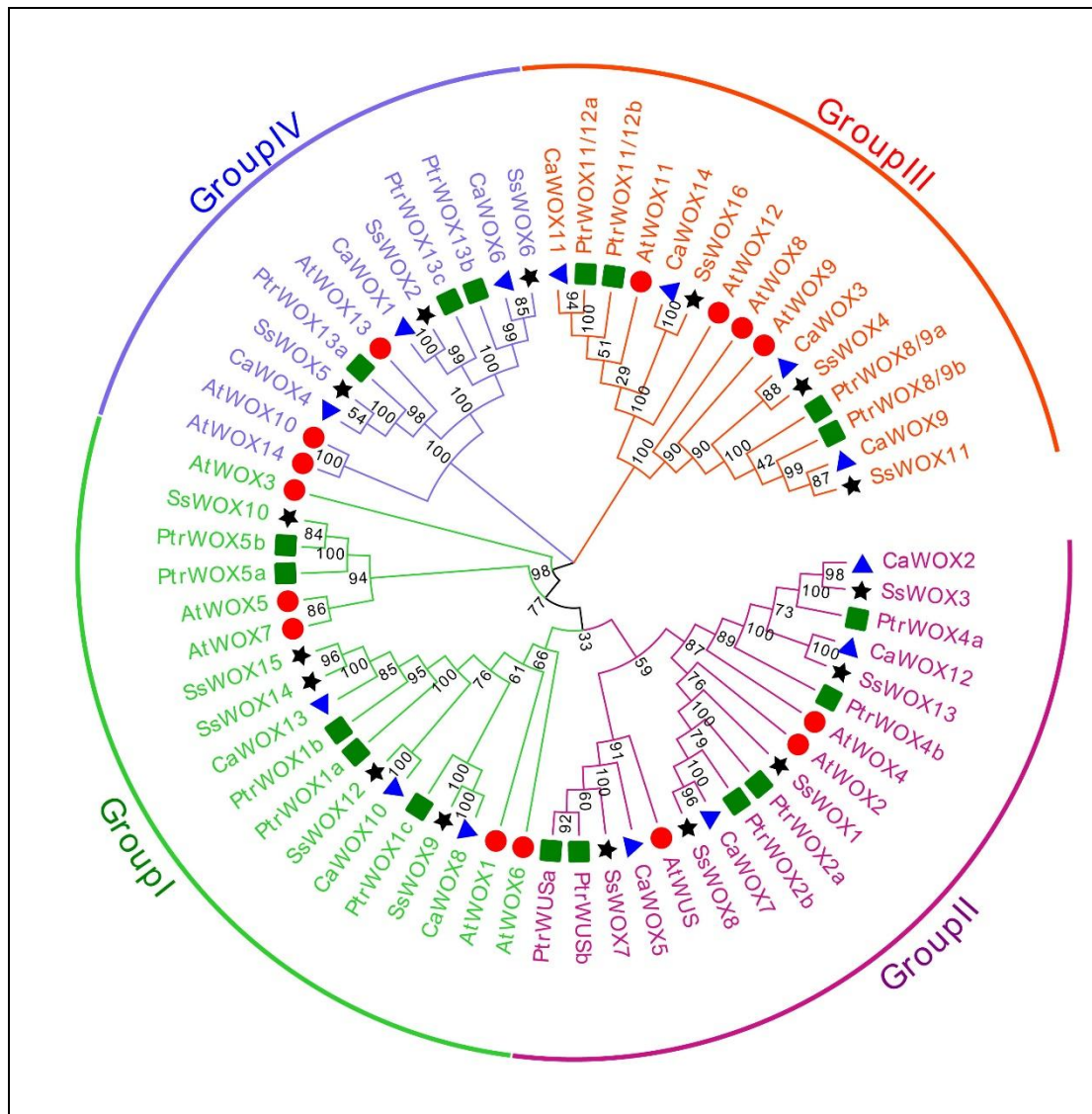
Figure 1. Phylogenetic tree of the WOX gene family across different species. The evolutionary relationships among WOX genes from A. thaliana , P. trichocarpa , C. arbutifolia , and S. suchowensis are shown.
