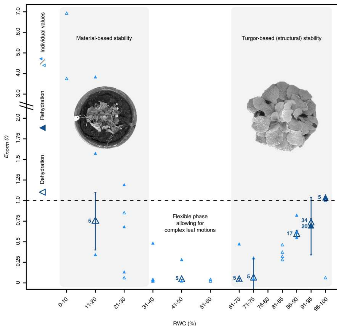
FIGURE 5 | Water status dependent alterations of the petiolar biomechanics of R. myconi . Dehydration (open triangles) induces a triphasic mechanical behavior, which is characterized by a turgor-based structural stability at high and a material-based stability at low water contents, and is fully reversible upon rehydration (closed triangles). The structural bending elastic moduli ( E ) have been normalized to the median bending modulus at RWCs > 90%. The normalized bending elastic moduli ( E_{norm} ) of each RWC interval are either given as median \pm standard error of the median ( N \geq 5 , large dark-blue symbols), or as individual values ( N < 5 , small light-blue symbols).
