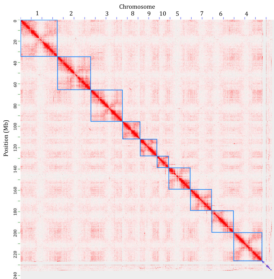
FIGURE 1 Hi-C based contig anchoring. Post-clustering heat map showing density of Hi-C interactions between contigs from the Juicer and 3d-DNA pipeline. The 10 Oropetium chromosomes are highlighted by blue squares
