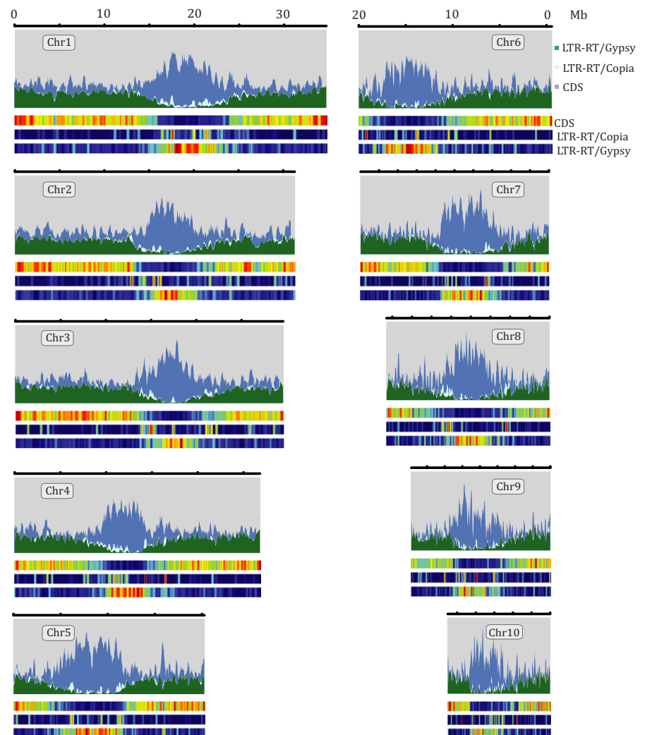
FIGURE 3 Landscape of the Oropetium genome. Gypsy and Copia long terminal repeat retrotransposons (LTR-RT) and CDS density are plotted for the 10 Oropetium chromosomes. Features are plotted in sliding windows of 50 kb with 25 kb step size. The location of centromere specific tandem arrays is highlighted by red bars. The heat maps below each landscape show relative density with red indicating high density and blue indicating low density for each feature
