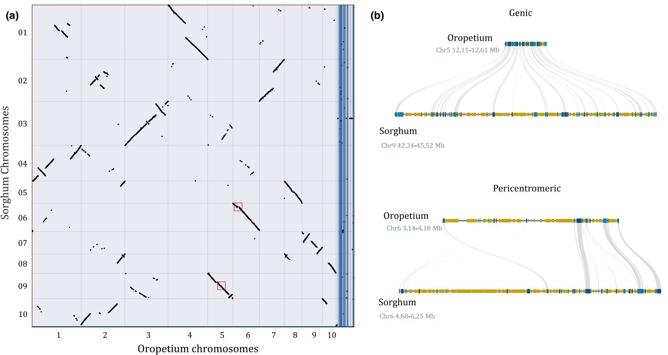
FIGURE 4 Comparative genomics between Oropetium and Sorghum . (a) Macrosyntentic dotplot of the Oropetium and Sorghum chromosomes based on 18,889 gene pairs. Each black dot represents a syntenic region between the two genomes. (b) Microsynteny of a typical genic region of Sorghum and Oropetium (top) and the pericentromeric region of Chromosome 6 of Oropetium and Sorghum (bottom). LTR-RTs are shown in yellow and genes are shown in blue. Syntenic orthologs are connected by gray lines. The centromeric repeat array in Oropetium is shown in red
