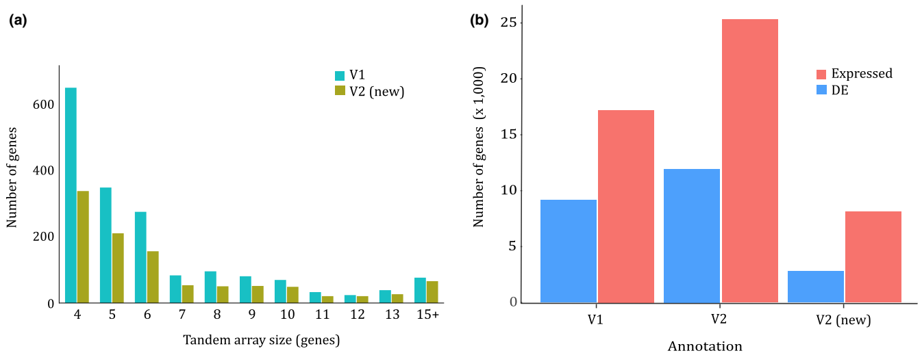
FIGURE 2 Characterization of the updated V2 Oropetium annotation. (a) Tandem gene array size comparison of the V1 and V2 annotation. Tandem genes identified in V1 are shown in blue and tandem genes newly annotated in V2 are shown in gold. (b) Comparison of expression patterns from the V1 and V2 annotation. The total number of genes with detectable expression and differential expression (DE) in the Oropetium desiccation/rehydration timecourse are plotted
