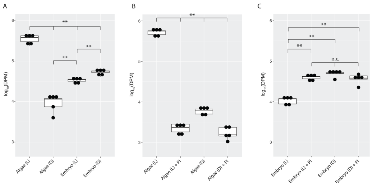
Figure 3. A. maculatum embryos compete with O. amblystomatis algae for bicarbonate. In each image, the y-axis represents radioactivity assayed per sample (DPM, disintegrations per minute); the x-axis represents the treatments. A. Algae from whole eggs incubated in the light (L) fixed significantly more carbon than algae in the dark (D) and embryos in the light or dark. Embryos in the light fixed more carbon than algae in the dark. Embryos in the dark fixed significantly more carbon than embryos in the light and algae in the dark. B. Photosynthesis inhibitors (PI) halt carbon fixation in algae in the light to a similar extent to keeping the algae in the dark. C. In the whole egg environment, photosynthesis inhibitors cause significantly increased carbon fixation in embryos, reproducing the effect seen when eggs are kept in the dark. n.s.=not significant, ** p < 0.01 . Significance levels were determined by ANOVA followed by the Games-Howell post-hoc test.
