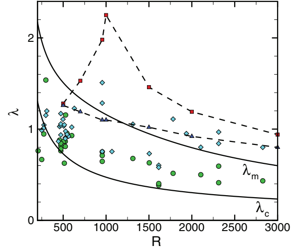
FIG. 8. (Color online) Variation of the wavelength of bioconvection \lambda with Rayleigh number R . The squares (red) are the long-time pattern wavelength from the numerical simulations (the patterns are shown in Fig. 6). The triangles (blue) are the short-time pattern wavelength from the numerical simulations. The dashed lines are included to guide the eye. The diamonds (cyan) and circles (green) are the experimentally measured short-time and long-time wavelengths, respectively, from Ref. [6]. The two labeled solid lines are the critical wavelength \lambda_c and the wavelength of maximum growth rate \lambda_m that have been determined from a linear stability analysis of a finite layer with an equilibrium base state and our boundary conditions.
