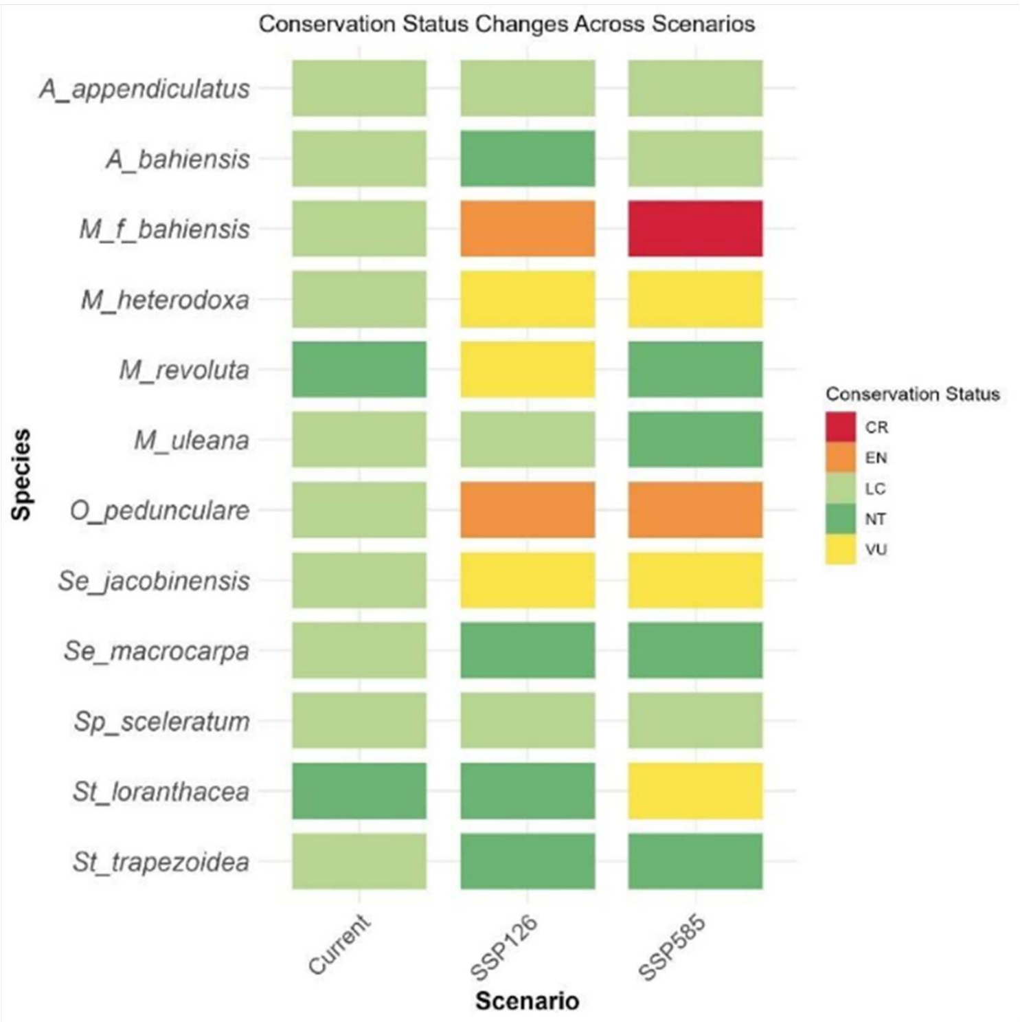
Figure 6 Conservation status projections of 12 endemic species of Northeastern Brazil under the current, optimistic (SSP126) and pessimistic (SSP585) climate scenarios
