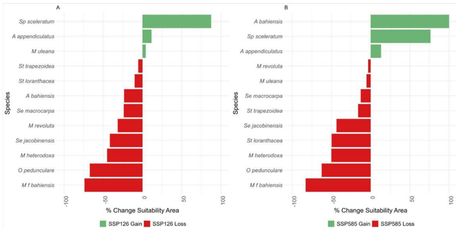
Figure 3 Percentage of loss and gain of environmental suitability area for endemic species under different climate scenarios: A = optimistic (SSP126); B = pessimistic (SSP585)
