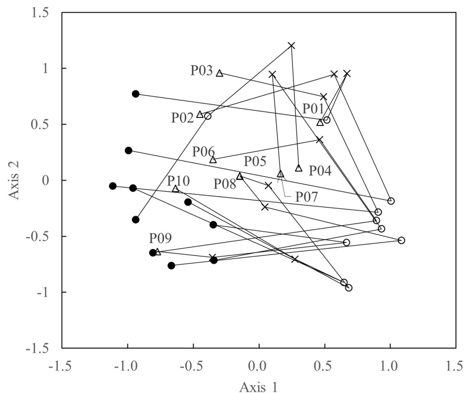
Figure 4 Scatterplots of the first two NMDS axes in each survey period. ● = 2008; ○ = 2018; × = 2019; △, 2020. “P01–10” = quadrat numbers. Full-size DOI: 10.7717/peerj.17487/fig-4
