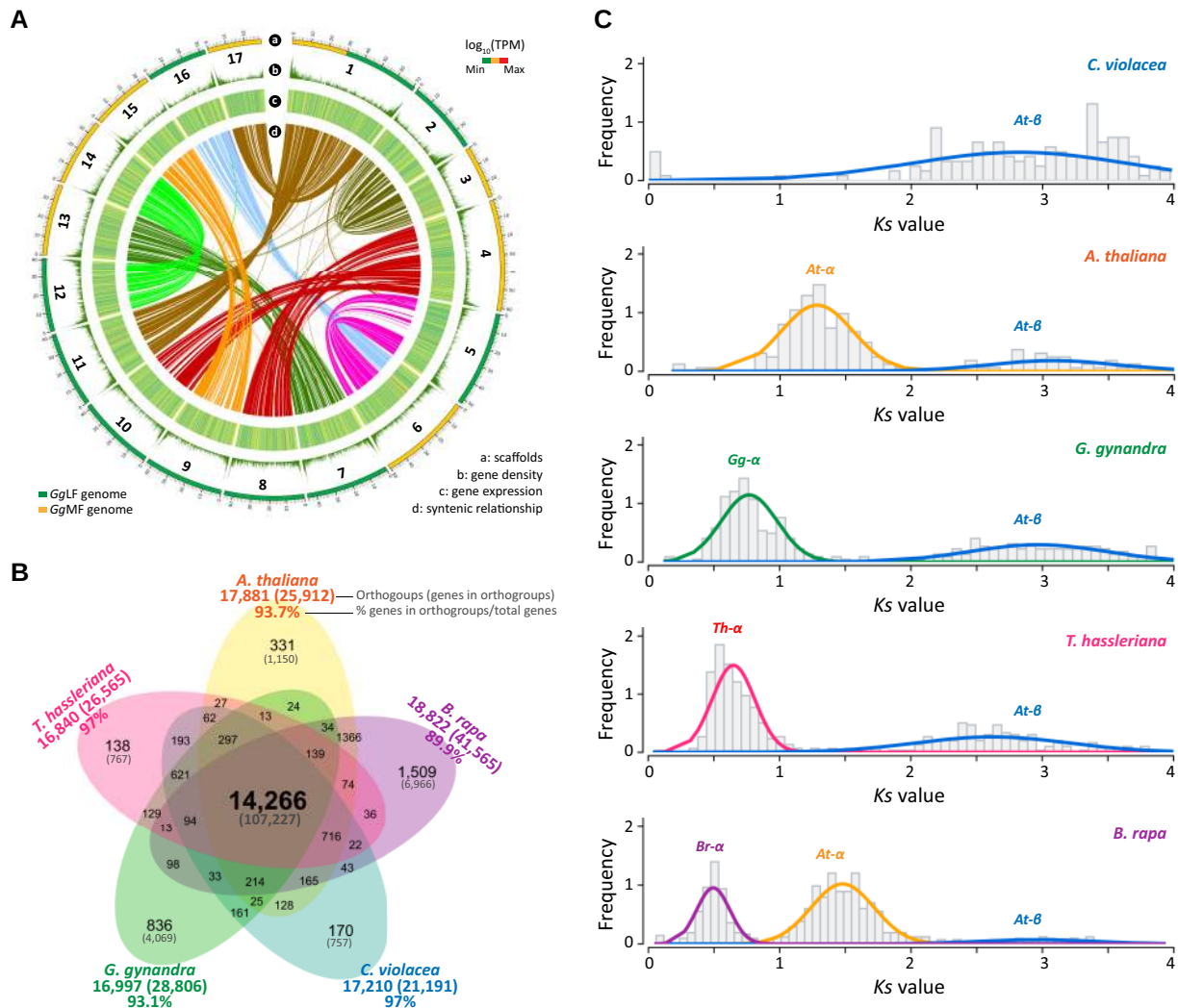
Figure 1 The genome sequence of G. gynandra , intraspecies synteny, gene orthogroup clustering, and whole-genome duplication events. A, Circos plot showing largest 17 pseudomolecules of the G. gynandra genome assembly (track a) including two subgenomes GgLF (green) and GgMF (yellow), gene density (track b), the expression level of the predicted gene models (track c), and intraspecies syntenic blocks ( minspan = 4 genes) among the scaffolds analyzed by MCScan (track d). Gene densities were estimated by a window of 100 kb. Gene expression was calculated for each window of 100 kb, using leaf developmental (stages Leaf_0 to Leaf_5) transcriptome data from K ulahoglu et al. (2014), quoted as log 10 (average TPM). Ribbon links in the inner track convey syntenic regions between two pseudomolecules and generally show a clear 2:2 syntenic pattern. Scaffold length is in Mb. B, Venn diagram illustrating the commonly shared and unique orthogroups from G. gynandra , C. violacea , T. hassleriana , A. thaliana , and B. rapa . Numbers in brackets denote the genes included in the orthogroups. Percentages were calculated based on the total genes annotated in each genome. C, Whole-genome duplication (WGD) events identified in different species by fitting the Ks distributions for WGD-derived gene pairs using Gaussian Mixture Models (GMMs). Ks peaks corresponding to At-β (commonly shared), At-α in A. thaliana and B. rapa , Gg-α in G. gynandra , Th-α in T. hassleriana and Br-α in B. rapa . Only Ks \leq 4 were included in this analysis.
