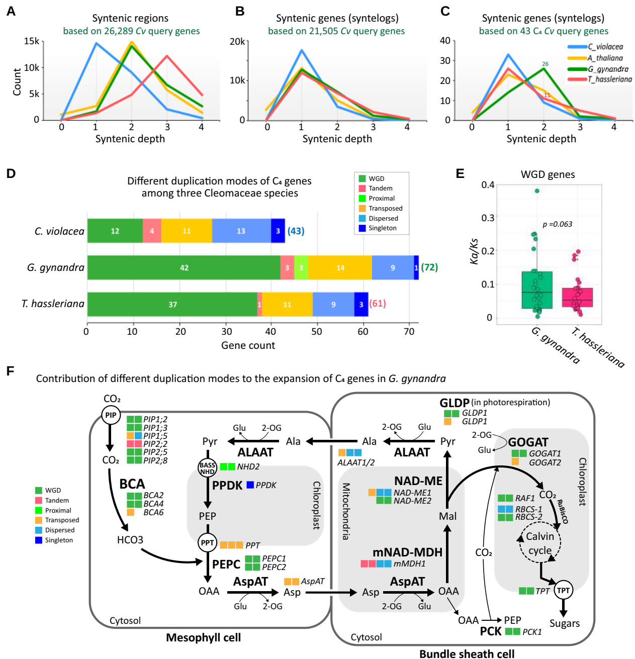
Figure 6 Contribution of gene duplication on the evolution of C 4 photosynthesis in Cleomaceae. A–C, Plots of syntenic regions and genes analyzed by SynFind using all C. violacea genes and a set of 43 genes known to be involved in C 4 photosynthesis, searched against the genomes of A. thaliana , G. gynandra , and T. hassleriana . For each panel, genes that showed no syntenic regions or syntelogs in both G. gynandra and T. hassleriana were excluded. D, Number of syntelogs identified in each species corresponding to the 43 C 4 genes in the C. violacea genome. Modes of gene duplication were obtained from the Dupgene_finder results presented in Figure 4. E, Ka/Ks ratios of WGD-derived gene pairs among the syntelogs identified in G. gynandra and T. hassleriana as shown in (D). The P-value was calculated by Student's two-sided t-test. F, Expansion pattern and duplication modes of gene families involved in C 4 photosynthesis. Each box represents one gene copy. Box colors indicate duplication mode that are shown at the bottom left corner. The expanded gene copies were derived from both SynFind analysis and Dupgene_finder results (in Figure 4). BCA (BETA CARBONIC ANHYDRASE), PEPC (PHOSPHOENOLPYRUVATE CARBOXYLASE), AspAT (ASPARTATE AMINOTRANSFERASE), mMDH (MITOCHONDRIAL MDH), NAD-ME (NAD-DEPENDENT MALIC ENZYME), ALAAT (ALANINE AMINOTRANSFERASE), PPDK (PYRUVATE ORTHOPHOSPHATE DIKINASE), PCK (PHOSPHOENOLPYRUVATE CARBOXYKINASE), GOGAT (GLUTAMINE OXOGLUTARATE AMINOTRANSFERASE), GLDP (GLYCINE DECARBOXYLASE P-PROTEIN), TPT (TRIOSE-PHOSPHATE/PHOSPHATE TRANSLOCATOR), PIPs (PLASMA MEMBRANE INTRINSIC PROTEIN), RBCS (RUBISCO SMALL SUBUNIT), RAF1 (RUBISCO ACCUMULATION FACTOR1), OAA (OXALOACETATE), Asp (ASPARTIC ACID), Mal (MALATE), Pyr (PYRUVATE), Ala (ALANINE), PEP (PHOSPHOENOLPYRUVATE), Glu (GLUTAMATE), and 2-OG (2-OXOGLUTARATE).
