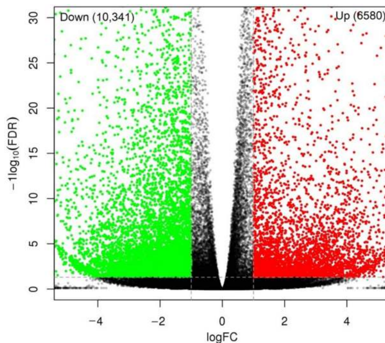
Figure 6. Volcano plot of unigenes and number of differentially expressed genes (DEGs) in the CR compared with CS.
