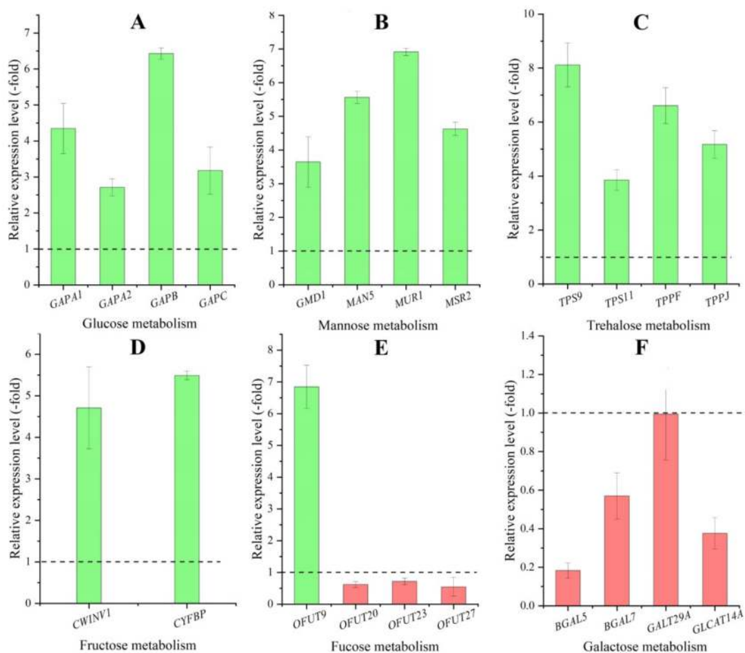
Figure 8. The relative expression level of genes involved in metabolism process of glucose (A), mannose (B), trehalose (C), fructose (D), fucose (E) and galactose (F) in the CR compared with CS, as determined by qRT-PCR. Column highlighted in green represents genes UR and red represents genes DR. The dotted line in the images differentiates UR (>1) and DR (<1) in CR compared with CS, represented. The same below.
