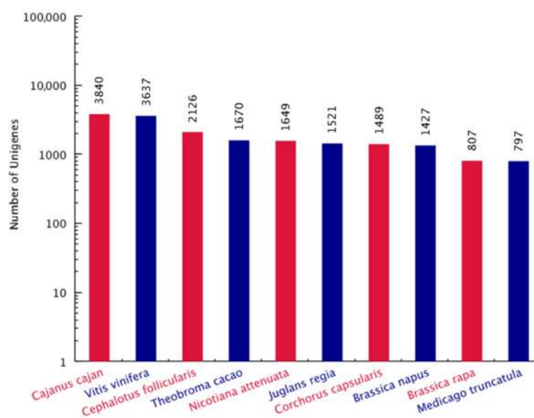
Figure 5. Top 10 species distribution of unigenes against Nr database.
