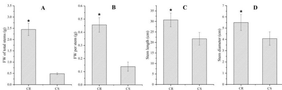
Figure 1. Growth characteristics of stems of Cynomorium songaricum host in Nitraria roborowskii (CR) and Cynomorium songaricum host in Nitraria sibirica (CS) (mean ± SD, n = 20). Images (A–D) represent FW of total stems, FW per stem, stem length and diameter, respectively. A t-test was applied for independent samples, the “*” is considered significant at p < 0.05 between CR and CS.
