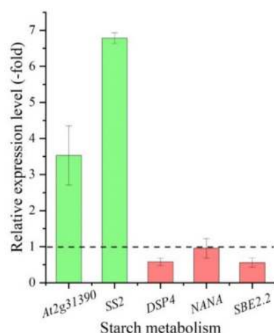
Figure 9. The relative expression level of genes involved in starch metabolism in the CR compared with CS, as determined by qRT-PCR.
