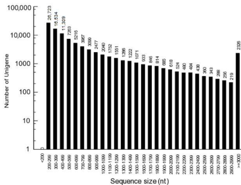
Figure 3. Length distribution of assembled unigenes in C. songaricum .
