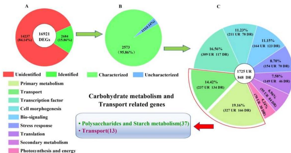
Figure 7. Distribution and classification of DEGs in the CR compared with CS (UR, up-regulation; DR, down-regulation). Image (A) represents the classification of unidentified and identified genes, image (B) represents the classification of uncharacterized and characterized genes and image (C) represents the classification of the functional genes.
