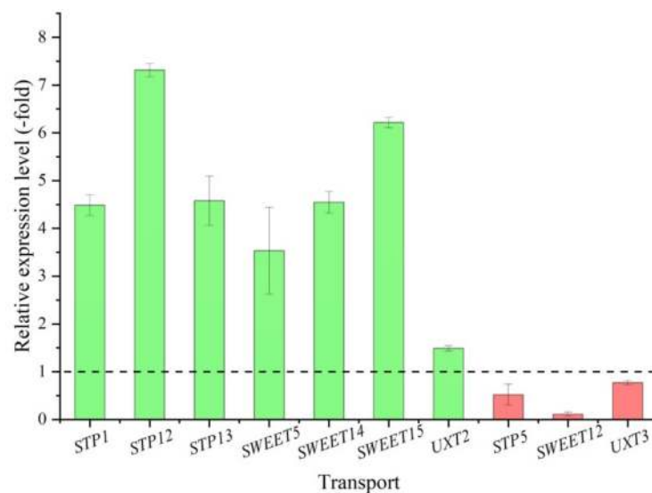
Figure 10. The relative expression level of genes involved in transport in the CR compared with CS, as determined by qRT-PCR.
