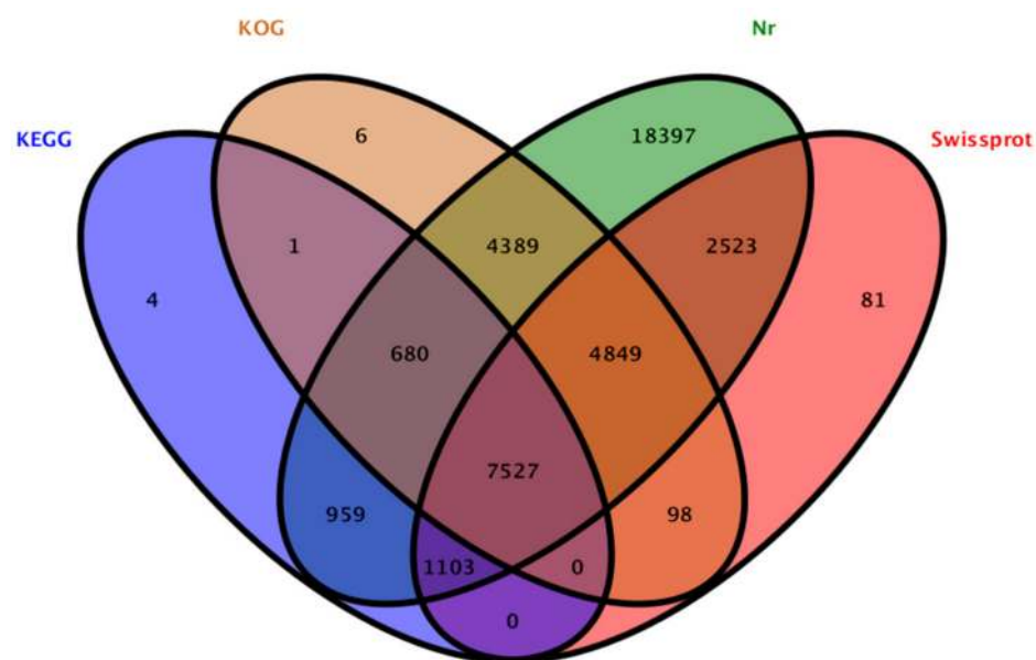
Figure 4. Basic annotation for all unigenes in C. songaricum on KEGG, KOG, Nr and Swissprot databases.
