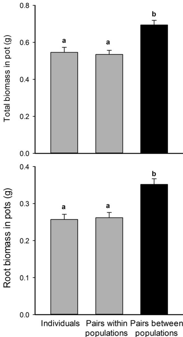
Figure 1. Total and root biomass in pots with either a P. spicata plant grown alone, grown with another plant of the same population or with a plant from a different population. Means that share a letter are not significantly different and error bars represent 1 SE.
