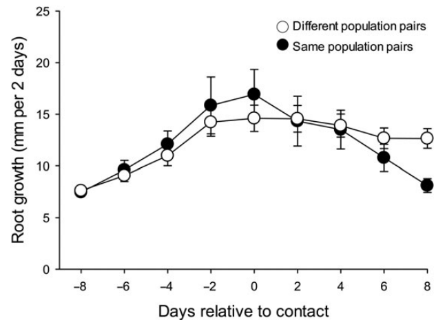
Figure 2. Rates of elongation of roots of P. spicata plants grown towards and making contact with roots of other P. spicata plants from either the same population or a different population. Elongation rates were standardized in time by aligning at Day 0 the days on which their contact with a target root was recorded (see Mahall and Callaway 1996). Error bars represent 1 SE.
