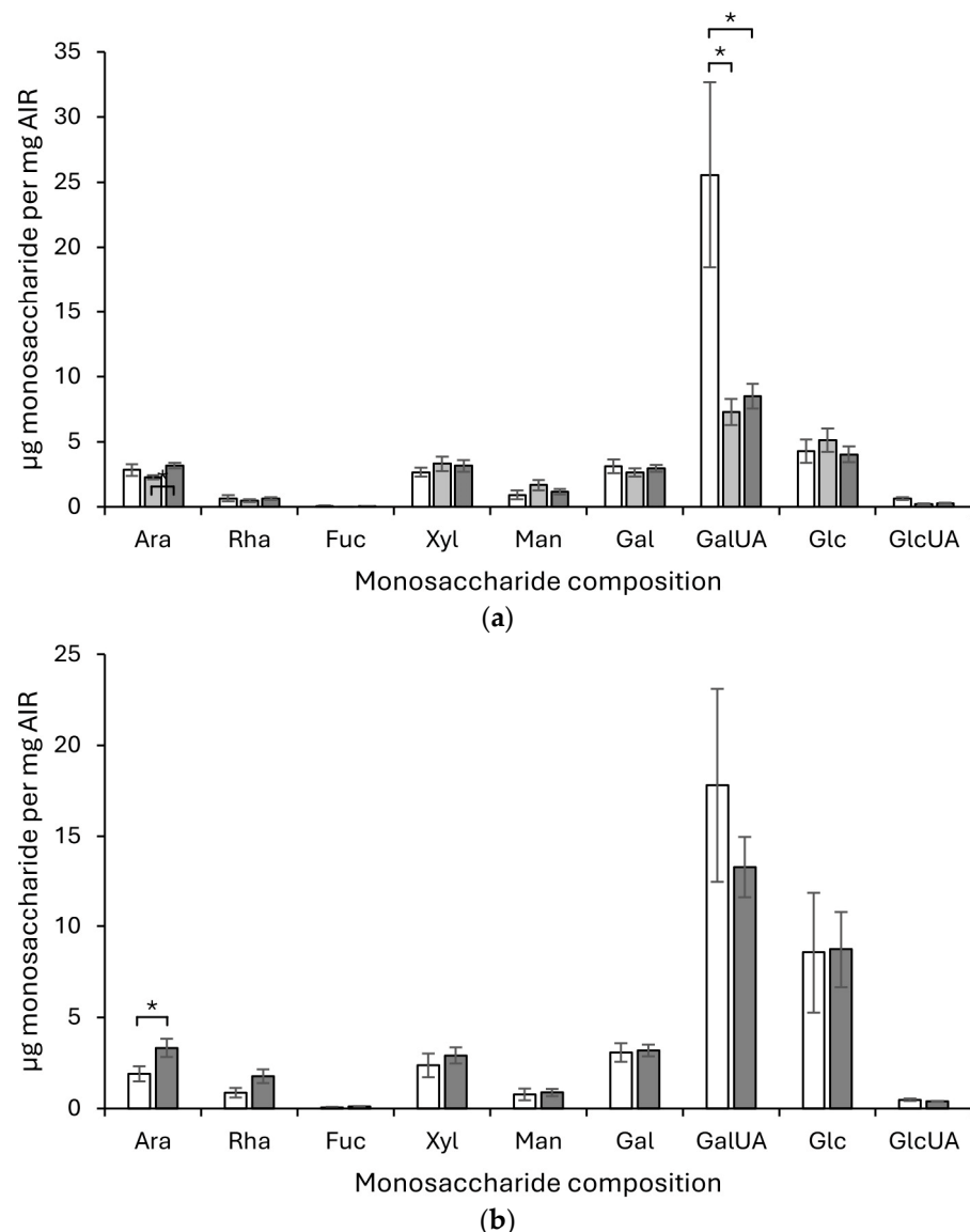
Figure 1. Monosaccharide compositional analysis of the total AIR isolated from leaf material of Craterostigma plantagineum (a), and Lindernia brevidens (b). White bars represent hydrated leaves, mid-grey shaded bars represent partially hydrated leaves and shaded bars represent desiccated leaves. Monosaccharide codes are for arabinose (Ara), rhamnose (Rha), fucose (Fuc), xylose (Xyl), mannose (Man), galactose (Gal), galacturonic acid (GalUA), glucose (Glc) and glucuronic acid (GlcUA). Error bars represent the standard error (SE) of the mean of four biological samples with two technical replicates per biological sample. Statistically significant differences, based on one-way ANOVA variance testing, are indicated on the bar graphs as an asterisk.
