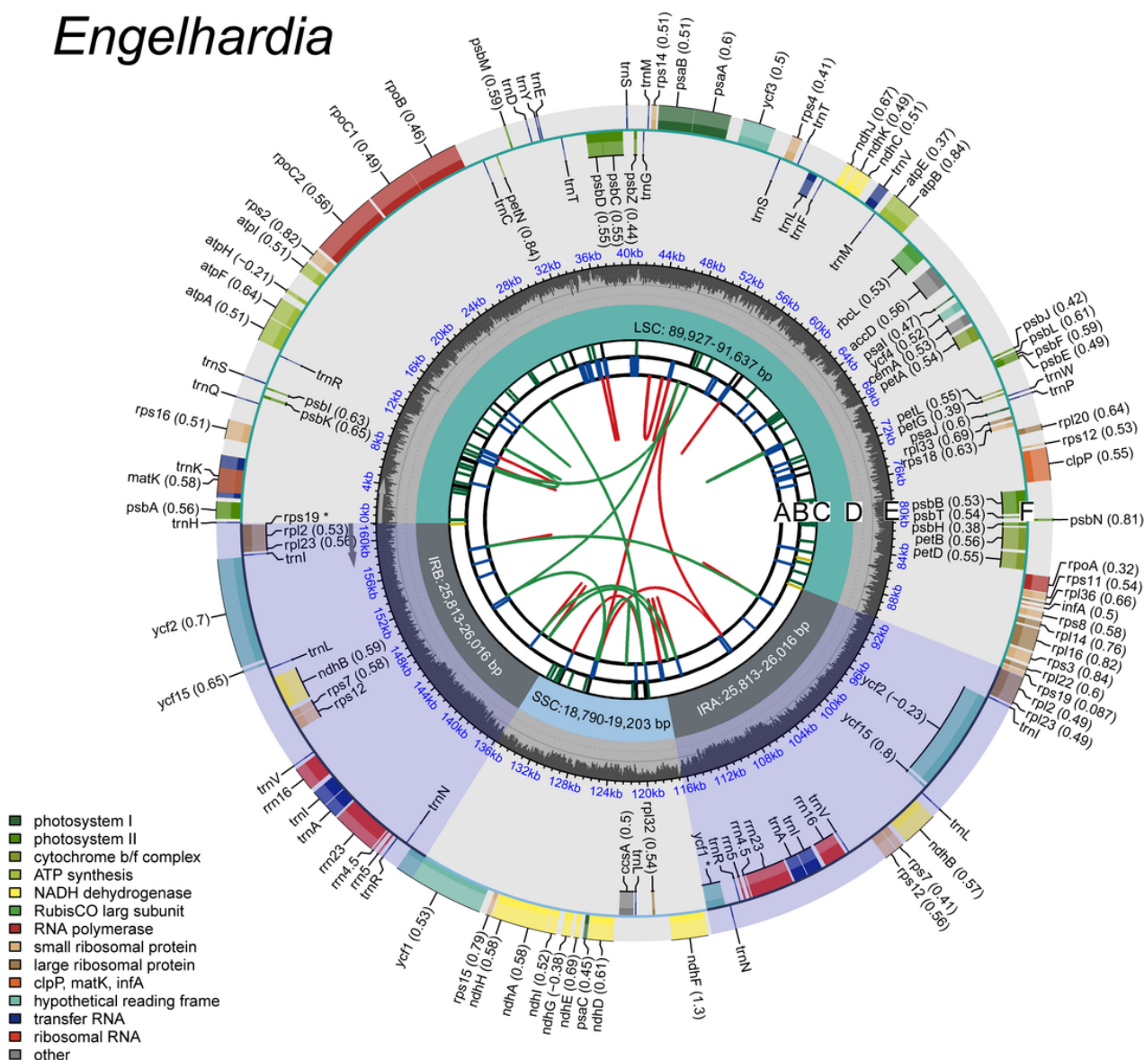
Figure 1 Gene map of Engelhardia plastomes. The species name is displayed in the upper left corner, and the genome map includes 5 tracks. From the inside out, the first track (A) displays forward and reverse repeats connected by red and green arcs. The second track (B) shows the tandem repeats, represented by blue line segments. The third track (C) displays the microsatellite sequences, represented by green
