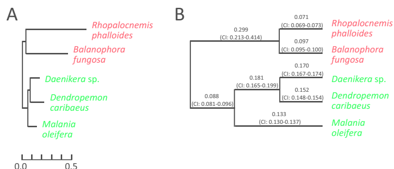
Figure 3 Evolutionary parameters of nuclear genes in the studied Santalales. (A) The phylogram where branch lengths represent numbers of substitutions per position. (B) The cladogram that depicts dN/dS values on branches with their 95% confidence intervals (CIs). Arabidopsis thaliana , used as the outgroup, is not shown. Names of non-photosynthetic species are in red, while names of photosynthetic species are in green. All bootstrap support values for the topology are 100%.
