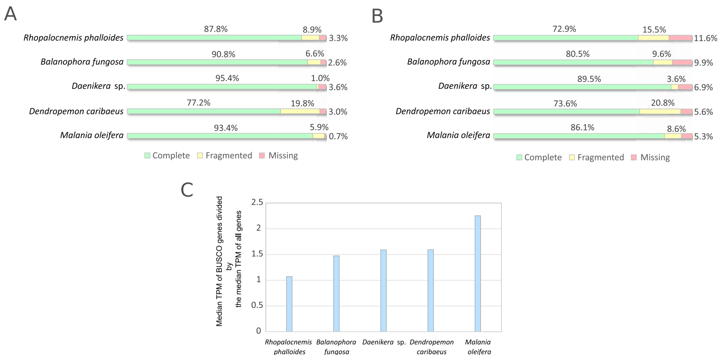
Figure 2 BUSCO analysis results. (A) BUSCO results for all sequences produced by Trinity. (B) BUSCO results for CDSs from major isoforms of transcripts after removal of transcripts with low coverage and contamination. (C) Comparison of expression of BUSCO genes and all genes. Full-size DOI: 10.7717/peerj.12106/fig-2
