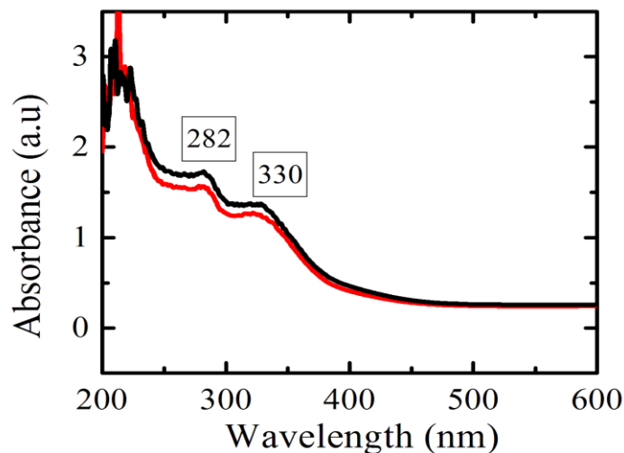
Fig.2. UV-Vis Absorption spectrum of biogenic CuNPs
