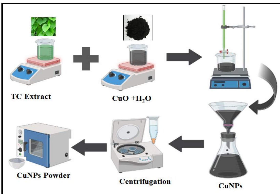
Fig.1. Biogenic Synthesis process of TC leaf extract mediated CuNPs
