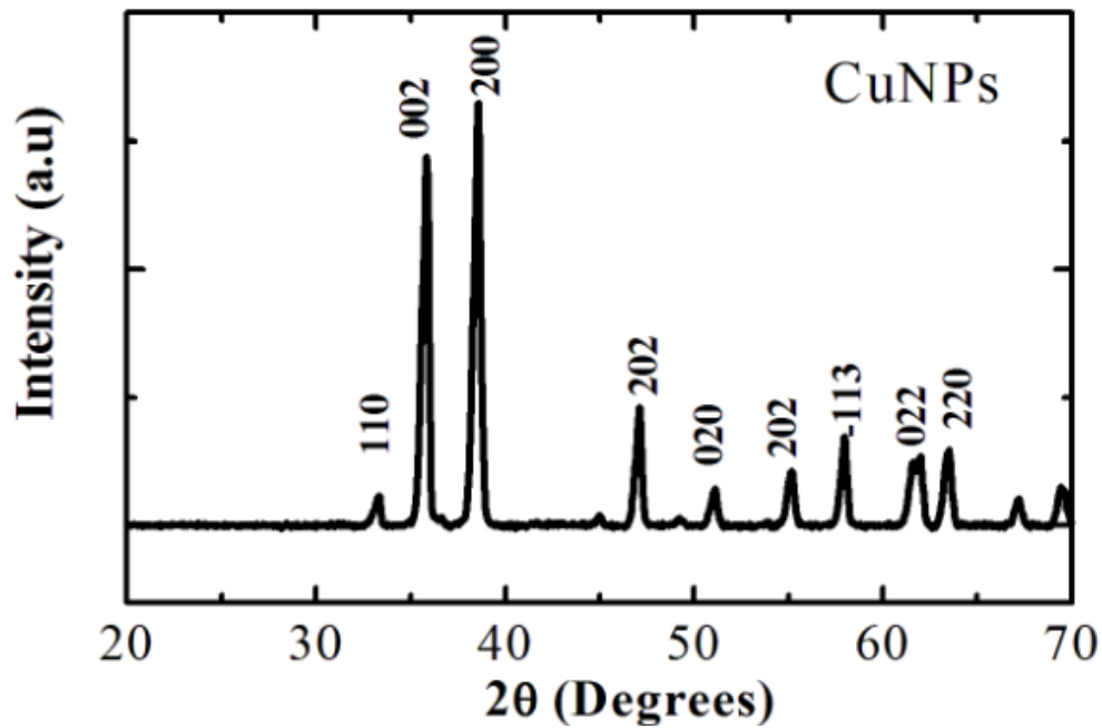
Fig.5. XRD pattern of CuNPs - JCPDS data card. 00-001-1117
