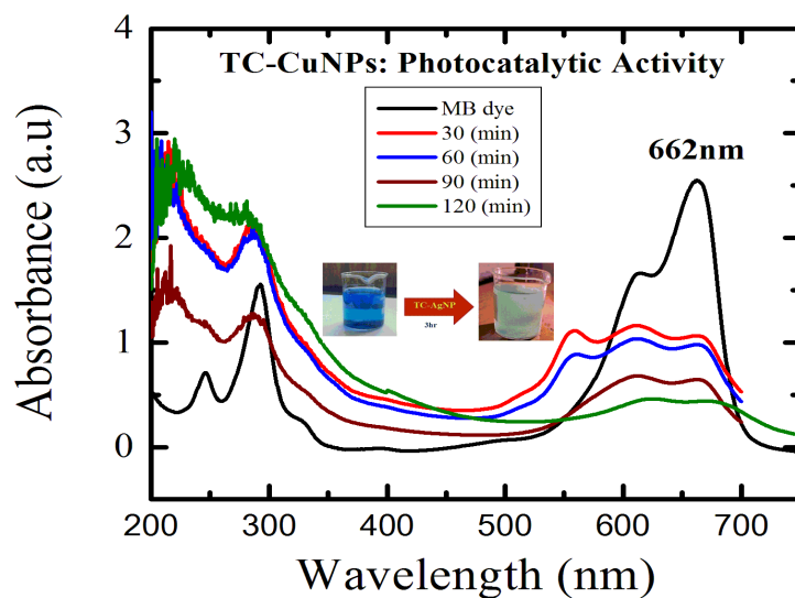
Fig.7. Absorption spectra of MB dye at different time intervals.
