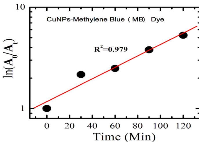
Fig.11. Kinetic results for dye degradation: \ln(A_t/A_0) vs Time
