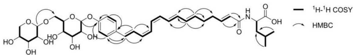
Figure 3. Key 1 H- 1 H COSY and HMBC correlations of compound 1.
