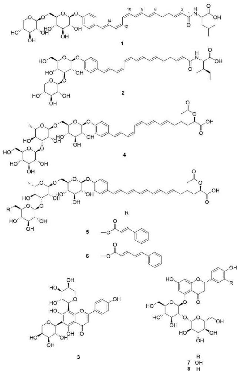
Figure 1. Chemical structures of compounds 1–3 isolated from R. franguloides and 4–8 previously isolated from B. berchemiifolia .
