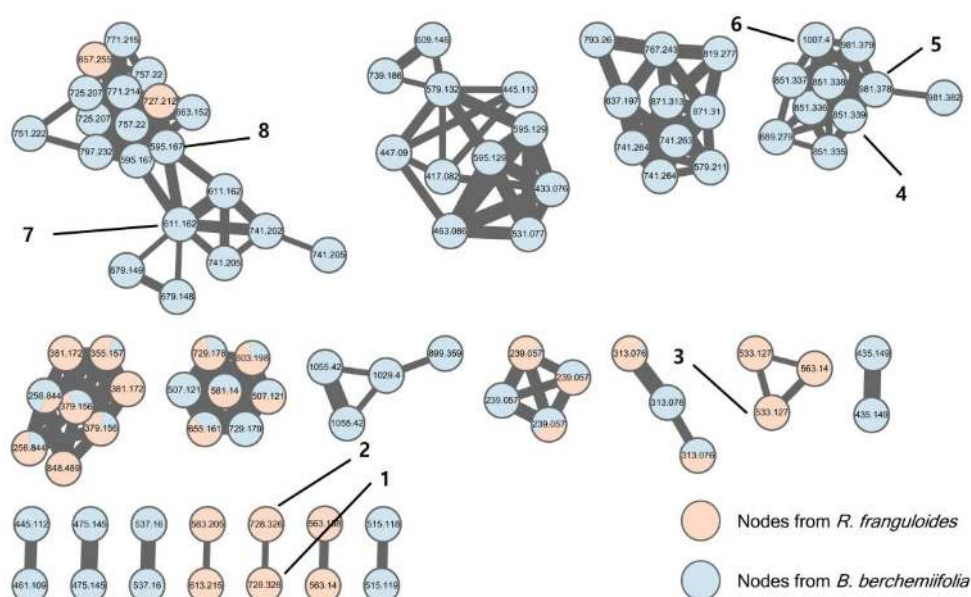
Figure 2. MS/MS molecular network of R. franguloides and B. berchemiifolia fruit extracts. Red nodes represent ions from R. franguloides ; blue nodes represent ions from B. berchemiifolia . Only clusters containing at least two nodes are shown.
