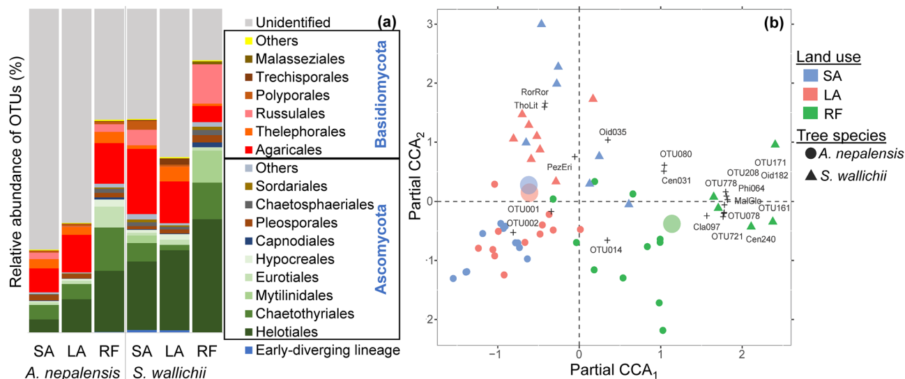
Fig. 4 a Relative abundance (%) of total fungi (at the order level) in A. nepalensis and S. wallichii among different types of land use. b Community composition of total fungi (variation explained by partial CCA 1 =4.8% and CCA 2 =3.25%) among different types of land use. Only the 20 most abundant OTUs are shown (abbreviation: MalGlo Malassezia globosa , PezEri Pezicula ericae , RorRor Roridomyces roridus , ThoLit Thozetella lithocarpis , Cen031 Cenococcum sp. 031,
