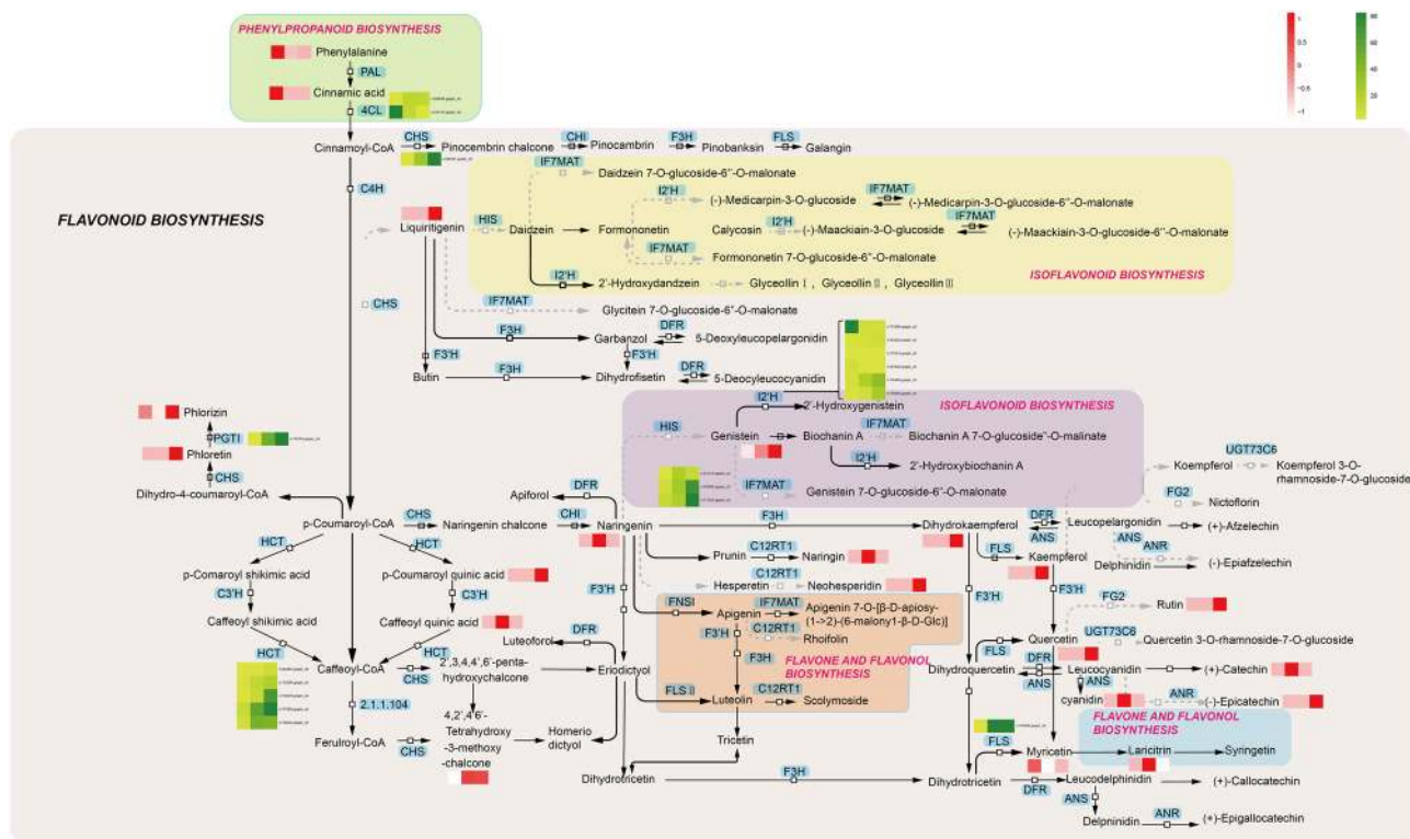
Figure 10. Visualization of protein and transcript expression in a biochemical pathway map related to flavonoid biosynthesis in G. pentaphyllum .
