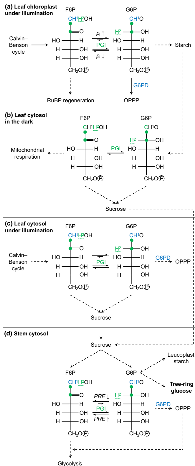
Fig. 5 Processes invoked to explain isotope fractionation at tree-ring glucose HC-1 and HC-2: (a) in leaf chloroplasts under illumination, (b) in the leaf cytosol in the dark, (c) in the leaf cytosol under illumination, and (d) in the stem cytosol. F6P and G6P carbon atoms 1–6 occur in sequentially order from top to bottom. Atom positions affected by G6PD and PGI fractionation are given in blue and green, respectively. In some cases, carbon position 1 is given both as blue letter and green dot to indicate fractionation at both enzymes. Dashed arrows indicate that intermediate reactions are not shown. Wavy lines indicate fractional introduction of hydrogen from water by the PGI reaction. Note that G6PD in stem leucoplasts may additionally contribute to isotope fractionation at tree-ring glucose C-1 and H 1 . F6P, fructose 6-phosphate; G6P, glucose 6-phosphate; G6PD, G6P dehydrogenase; OPPP, oxidative pentose phosphate pathway; PGI, phosphoglucose isomerase; p_i , intercellular CO 2 partial pressure; PRE, precipitation; RuBP, ribulose 1,5-bisphosphate.
