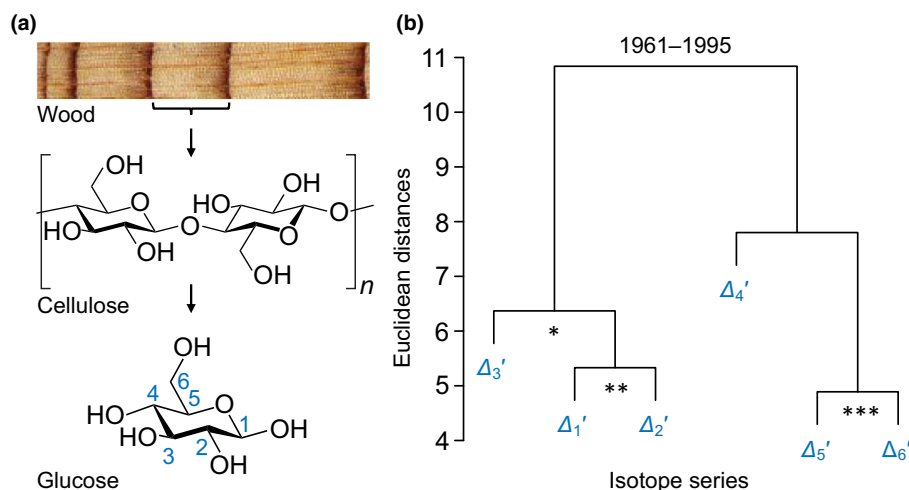
Fig. 1 Carbon isotope discrimination in tree rings. (a) Levels of resolution of stable carbon isotope analysis: whole plant materials, whole molecules, intramolecular carbon positions. (b) Hierarchical clustering of \Delta'_i series for the period 1961–1995. Significance of series correlation: *, P \leq 0.05 ; **, P \leq 0.01 ; ***, P \leq 0.001 . Modified figure from Wieloch et al. (2018). \Delta'_i denotes intramolecular ^{13}\text{C} discrimination in glucose extracted across an annually resolved Pinus nigra tree-ring series.
