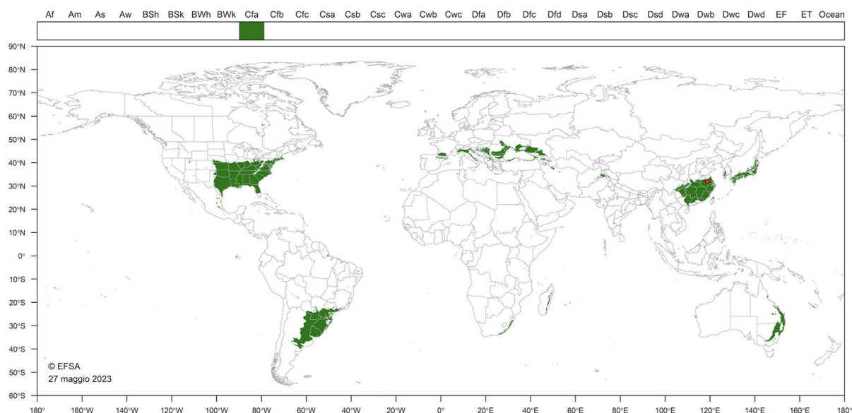
Figure 2: Occurrence of the Köppen–Geiger Cfa-climate type (humid subtropical climate) worldwide
