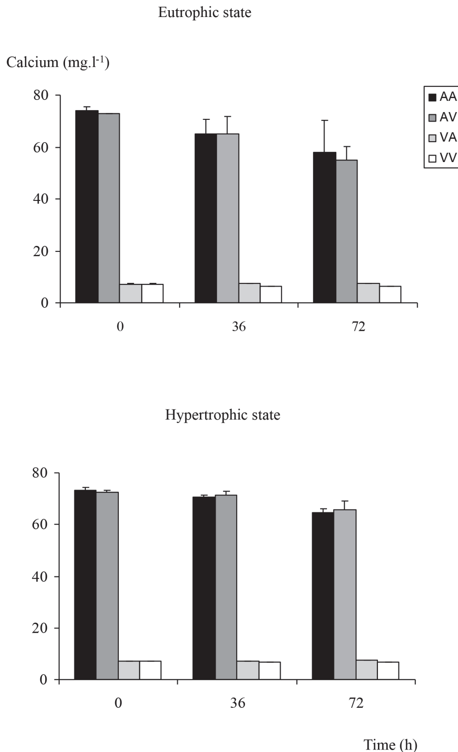
Fig 1. Dynamics of water calcium. Dynamics of calcium (in \text{mg.l}^{-1} ) contained in Alsatian or Vosgian water for eutrophic and hypertrophic conditions and for all the possible combinations of water and subpopulation. In the legend, AA, AV, VA, VV include the information on the treatment, the first letter refers to the type of water and the second one to the subpopulation (e.g. AV means Alsatian water and Vosgian subpopulation).
