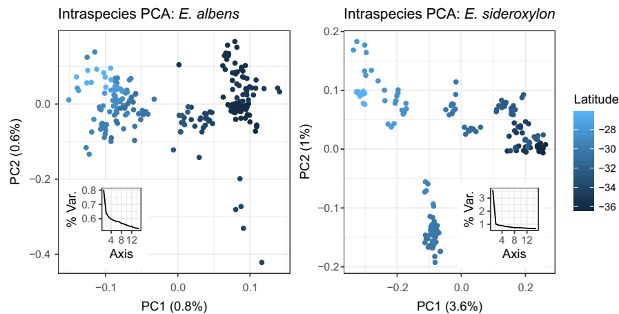
FIGURE 5 Principal component analysis (PCA) of Eucalyptus albens and E. sideroxylon individual genotypes. Axes describe eigendecomposition of PCANGSD estimates of sample covariance. Individuals are coloured by latitude, the primary axis of variation in species' distributions. Insets show the distribution of leading eigenvalues. Note the absence of strong discrete clusters, the strong trend in PC1 across latitude and the low proportion of genetic variance explained by each leading axis. We plot PC1 across a map of the study area for both species in Figure S13 and equivalent biplots with PC1, PC2 and PC3 in Figure S14 [Colour figure can be viewed at wileyonlinelibrary.com ]
