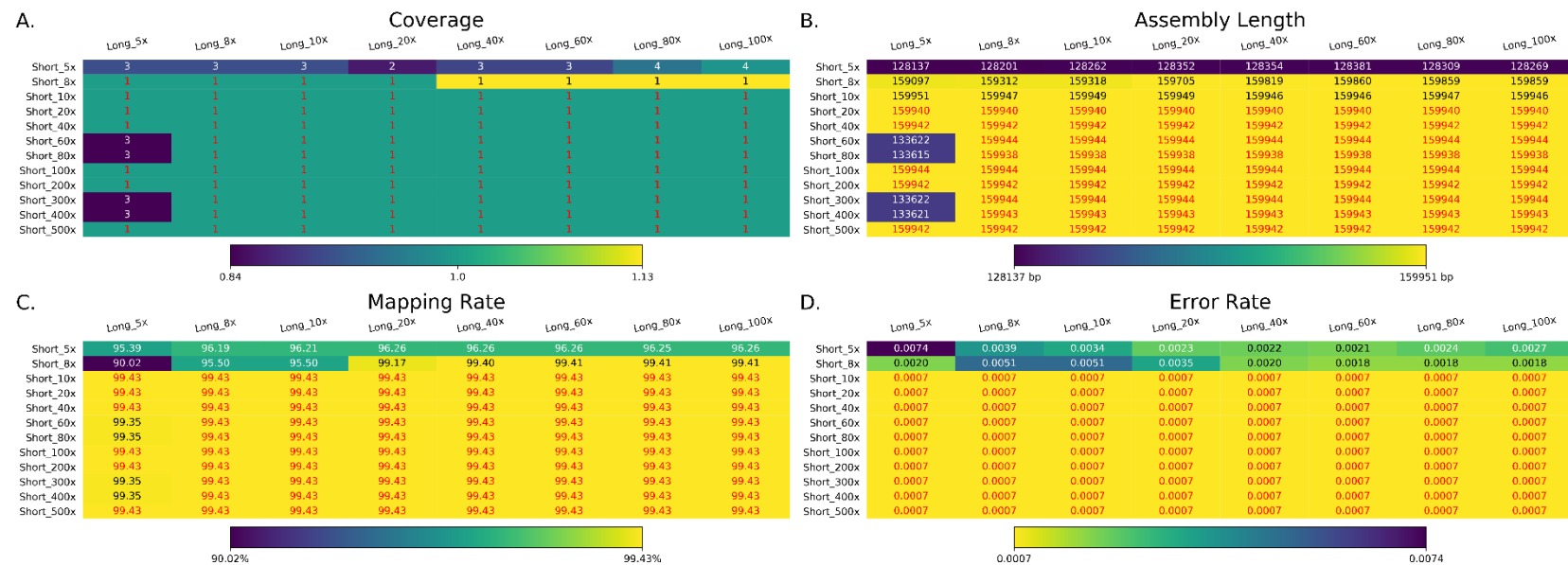
Figure S10. The summary of assemblies with Karect corrected short-reads and 40-50 kb long-reads. Long and Short indicate the coverage of this assembly. A. The total coverage of the chloroplast genome across all contigs output by the assembler. The number is the number of contigs of each assembly, whereas the heatmap is the genome coverage (it could be over 100% if some duplications exist). Numbers marked with red contained a single contig covering the whole chloroplast genome. The heatmap color is reversed compared to the Figure 1 to make the color in all figure panel A show consistence. B. The assembly length of different assemblies after manual curation (e.g. removing duplicate regions). Numbers marked with red denote assemblies with the expected length, in the range 155,938 bp–155,945 bp. C. The mapping rate of validation reads to the assemblies after manual curation. Assemblies with highest mapping rate (99.43%) are marked with red. D. The average per-base error rate of validation reads mapped to each manually-curated genome assembly. Assemblies with the lowest error rate (0.0007) are marked with red.
