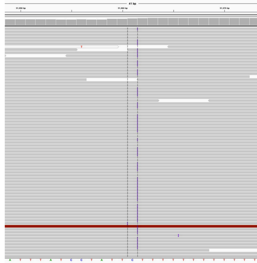
Figure S12. The long-/short-read mapping coverage in the possible heteroplastic site 51961 (IGV view). The purple “I” in short-reads indicated the T insertion, whereas the black lines in long-reads indicate the deletion during that region.
