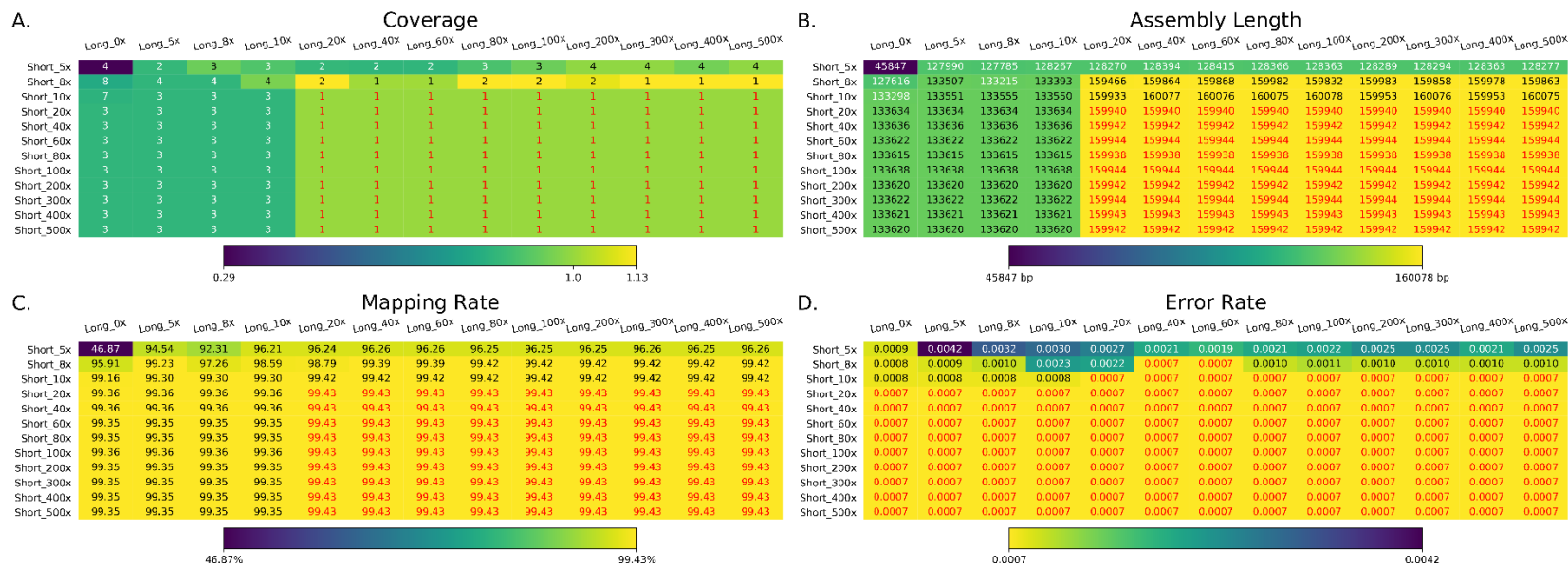
Figure S4. The summary of short-read-only and hybrid assemblies with Karect+SPAdes short-read correction. Long and Short indicate the coverage of this assembly. A. The total coverage of the chloroplast genome across all contigs output by the assembler. The number is the number of contigs of each assembly, whereas the heatmap is the genome coverage (it could be over 100% if some duplications exist). Numbers marked with red contained a single contig covering the whole chloroplast genome. The heatmap color is reversed compared to the Figure 1 to make the color in all figure panel A show consistence. B. The assembly length of different assemblies after manual curation (e.g. removing duplicate regions). Numbers marked with red denote assemblies with the expected length, in the range 155,938 bp–155,945 bp. C. The mapping rate of validation reads to the assemblies after manual curation. Assemblies with highest mapping rate (99.43%) are marked with red. D. The average per-base error rate of validation reads mapped to each manually-curated genome assembly. Assemblies with the lowest error rate (0.0007) are marked with red.
