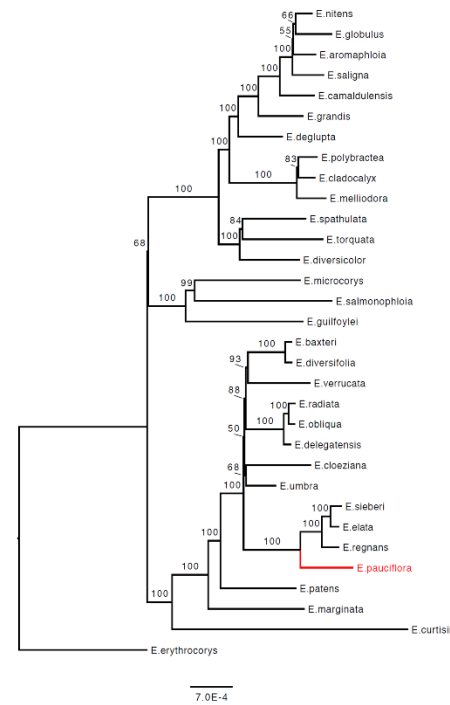
Fig 3. A. Annotated E. pauciflora chloroplast genome. Genes shown on the inside of the circle are transcribed clockwise, whereas genes shown on the outside of the circle transcribed counterclockwise. The grey region in the inside circle shows the GC content across the chloroplast genome. This figure was produced by OGDraw v1.2 [88]. B. A phylogenetic tree of 32 Eucalyptus taxa based on analysis of full chloroplast genomes.
