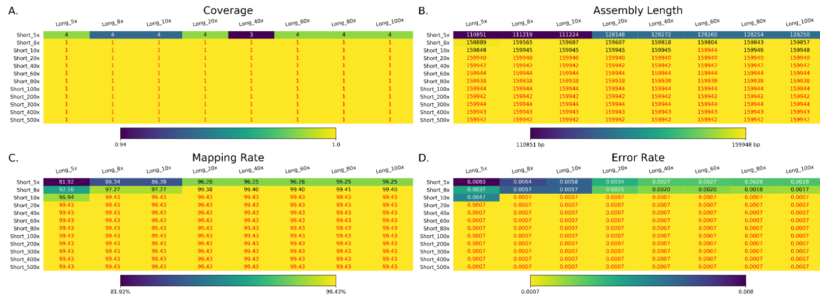
Figure S11. The summary of assemblies with Karect corrected short-reads and \geq 50 kb long-reads. Long and Short indicate the coverage of this assembly. A. The total coverage of the chloroplast genome across all contigs output by the assembler. The number is the number of contigs of each assembly, whereas the heatmap is the genome coverage (it could be over 100% if some duplications exist). Numbers marked with red contained a single contig covering the whole chloroplast genome. The heatmap color is reversed compared to the Figure 1 to make the color in all figure panel A show consistence. B. The assembly length of different assemblies after manual curation (e.g. removing duplicate regions). Numbers marked with red denote assemblies with the expected length, in the range 155,938 bp–155,945 bp. C. The mapping rate of validation reads to the assemblies after manual curation. Assemblies with highest mapping rate (99.43%) are marked with red. D. The average per-base error rate of validation reads mapped to each manually-curated genome assembly. Assemblies with the lowest error rate (0.0007) are marked with red.
