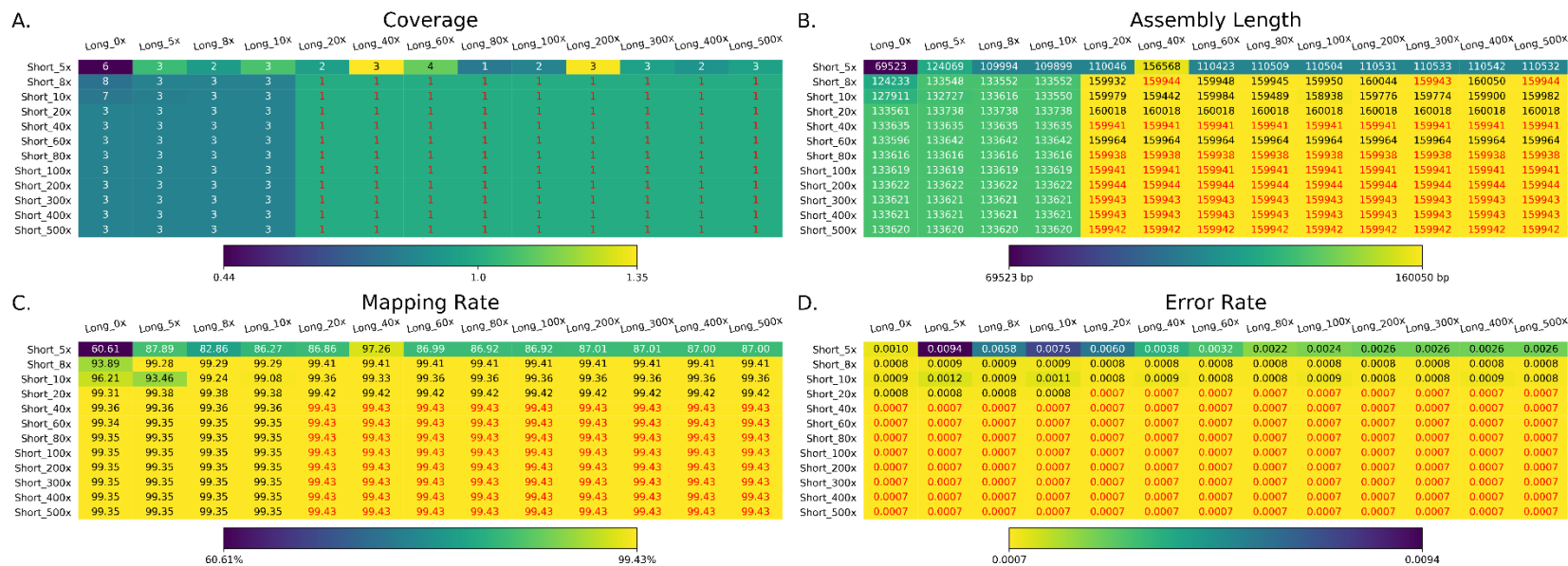
Figure S3. The summary of short-read-only and hybrid assemblies with SPAdes short-read correction. Long and Short indicate the coverage of this assembly. A. The total coverage of the chloroplast genome across all contigs output by the assembler. The number is the number of contigs of each assembly, whereas the heatmap is the genome coverage (it could be over 100% if some duplications exist). Numbers marked with red contained a single contig covering the whole chloroplast genome. The heatmap color is reversed compared to the Figure 1 to make the color in all figure panel A show consistence. B. The assembly length of different assemblies after manual curation (e.g. removing duplicate regions). Numbers marked with red denote assemblies with the expected length, in the range 155,938 bp–155,945 bp. C. The mapping rate of validation reads to the assemblies after manual curation. Assemblies with highest mapping rate (99.43%) are marked with red. D. The average per-base error rate of validation reads mapped to each manually-curated genome assembly. Assemblies with the lowest error rate (0.0007) are marked with red.
