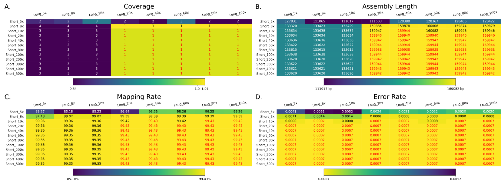
Figure S8. The summary of assemblies with Karect corrected short-reads and 20-30 kb long-reads. Long and Short indicate the coverage of this assembly. A. The total coverage of the chloroplast genome across all contigs output by the assembler. The number is the number of contigs of each assembly, whereas the heatmap is the genome coverage (it could be over 100% if some duplications exist). Numbers marked with red contained a single contig covering the whole chloroplast genome. The heatmap color is reversed compared to the Figure 1 to make the color in all figure panel A show consistence. B. The assembly length of different assemblies after manual curation (e.g. removing duplicate regions). Numbers marked with red denote assemblies with the expected length, in the range 155,938 bp–155,945 bp. C. The mapping rate of validation reads to the assemblies after manual curation. Assemblies with highest mapping rate (99.43%) are marked with red. D. The average per-base error rate of validation reads mapped to each manually-curated genome assembly. Assemblies with the lowest error rate (0.0007) are marked with red.
