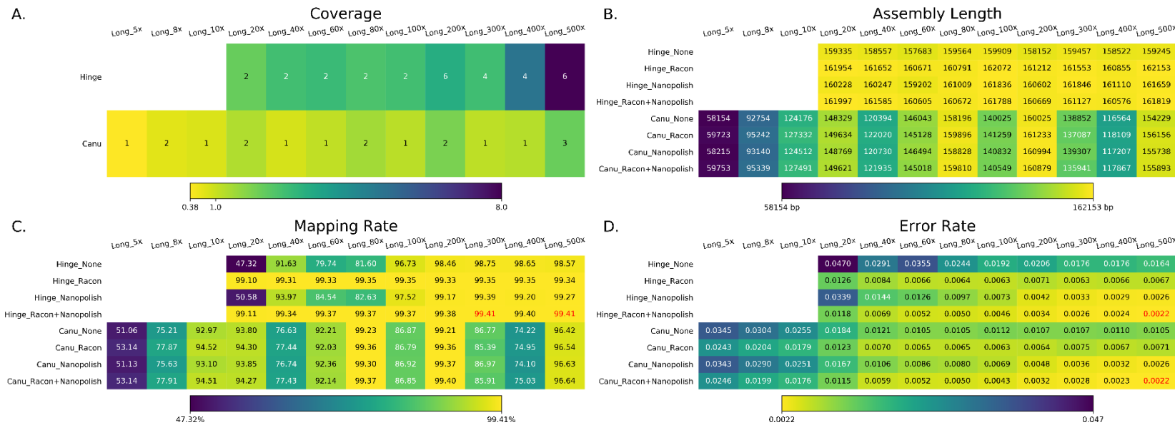
Figure S1. The summary of long-read-only assemblies. Long_5x indicates the 5x coverage of long-read was used in the assembly. Hinge failed to assemble genome with <20x coverage. None, Racon, Nanopolish and Racon+Nanopolish mean the different genome polishing pipeline. A. The total coverage of the chloroplast genome across all contigs output by the assembler. The number is the number of contigs of each assembly, whereas the heatmap is the genome coverage (it could be over 100% if some duplications exist). B. The assembly length of different assemblies after manual curation (e.g. removing duplicate regions). C. The mapping rate of validation reads to the assemblies after manual curation. D. The average per-base error rate of validation reads mapped to each manually-curated genome assembly.
