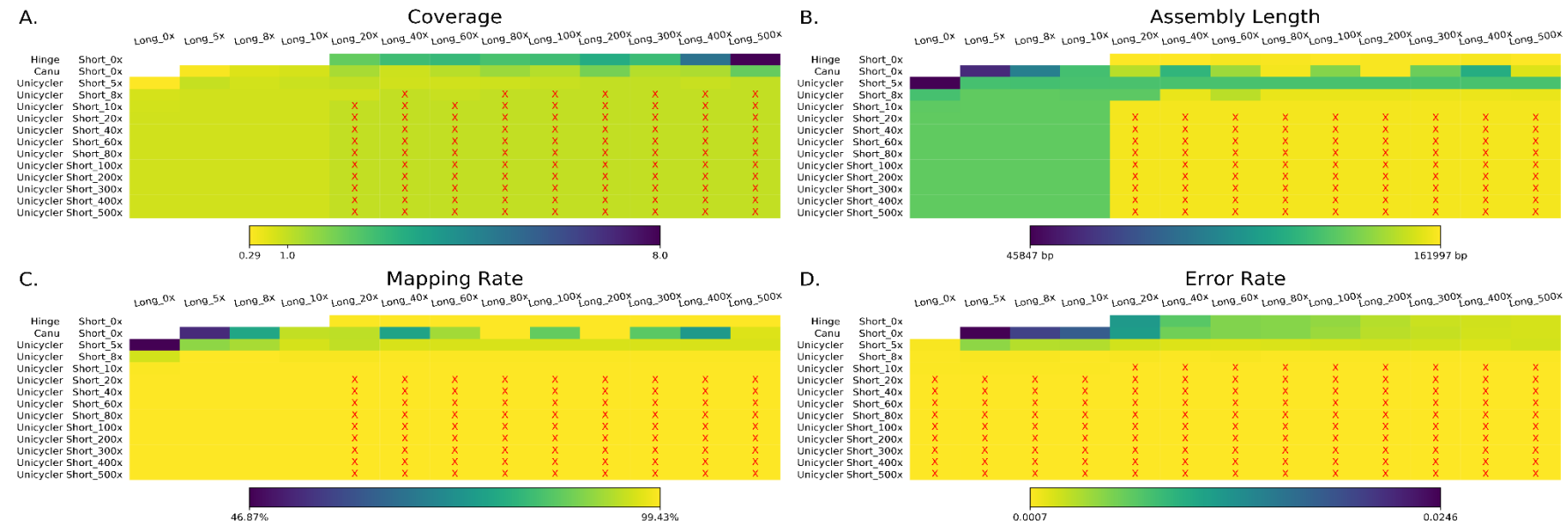
833 834 Fig 1. Comparison of chloroplast genome assemblies. The coverage of the long- and short-reads is shown along the top and left-hand-side of each panel, 835 respectively. The left-hand-side also shows which assembler was used for each row of assemblies in that panel. Hinge and Canu are long-read-only 836 assemblers, whereas Unicycler is short-read-only and hybrid assembler. The Hinge and Canu results in B, C, D were polished by Racon+Nanopolish, and the 837 Unicycler results used Karect-corrected short-reads. A. The total coverage of the chloroplast genome across all contigs output by the assembler. Panels 838 marked with a red 'x' contained a single contig covering the whole chloroplast genome. The heatmap indicates the chloroplast genome coverage. B. The 839 assembly length of different assemblies after manual curation (e.g. removing duplicate regions). Panels marked with an 'x' denote assemblies with the 840 expected length, in the range 155,938 bp–155,945 bp. C. The mapping rate of validation reads to the assemblies after manual curation. Assemblies with 841 highest mapping rate (99.43%) are marked with a red 'x'. D. The average per-base error rate of validation reads mapped to each manually-curated genome 842 assembly. Assemblies with the lowest error rate (0.0007) are marked with a red 'x'.
