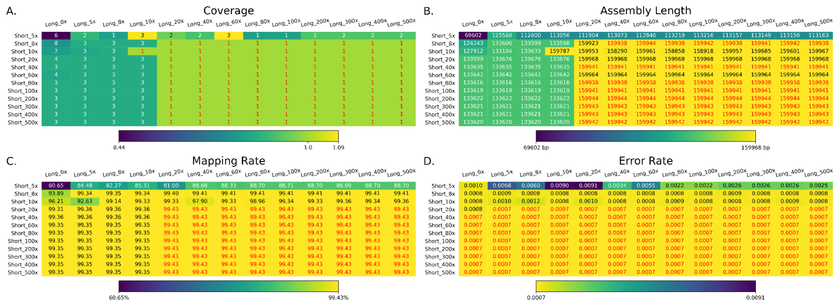
Figure S5. The summary of short-read-only and hybrid assemblies without any short-read correction. Long and Short indicate the coverage of this assembly. A. The total coverage of the chloroplast genome across all contigs output by the assembler. The number is the number of contigs of each assembly, whereas the heatmap is the genome coverage (it could be over 100% if some duplications exist). Numbers marked with red contained a single contig covering the whole chloroplast genome. The heatmap color is reversed compared to the Figure 1 to make the color in all figure panel A show consistence. B. The assembly length of different assemblies after manual curation (e.g. removing duplicate regions). Numbers marked with red denote assemblies with the expected length, in the range 155,938 bp–155,945 bp. C. The mapping rate of validation reads to the assemblies after manual curation. Assemblies with highest mapping rate (99.43%) are marked with red. D. The average per-base error rate of validation reads mapped to each manually-curated genome assembly. Assemblies with the lowest error rate (0.0007) are marked with red.
