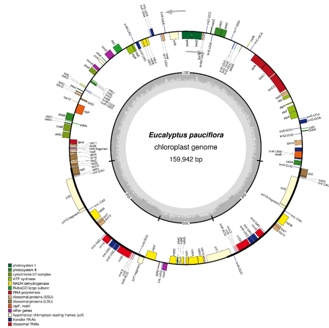
Fig 3. A. Annotated E. pauciflora chloroplast genome. Genes shown on the inside of the circle are transcribed clockwise, whereas genes shown on the outside of the circle transcribed counterclockwise. The grey region in the inside circle shows the GC content across the chloroplast genome. This figure was produced by OGDraw v1.2 [88]. B. A phylogenetic tree of 32 Eucalyptus taxa based on analysis of full chloroplast genomes.
