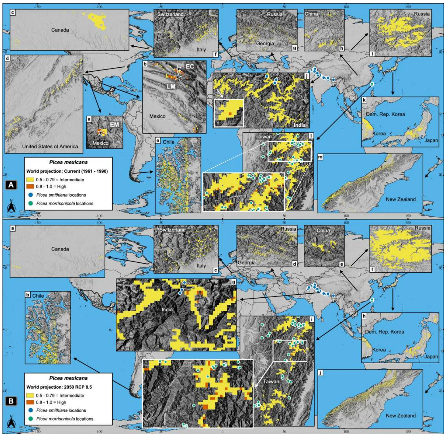
Figure 7 Global projections of the potential distribution of the climatically suitable habitat for Picea mexicana in contemporary conditions (A) and 2050 (B). All sites for the contemporary projection are located in many mountainous regions of the world, such as: Sierra Madre Occidental (A-a), Sierra Madre Oriental (A-b), Laurentian mountains (A-c), Appalachian Mountains (A-d), southern Andes (A-e), The Pyrenees (not shown), The Alps (A-f), the Caucasus mountains (A-g), Khingan mountains (A-h), Sayan mountains (A-i), The Himalayas (A-j), Sobaek-Taebaek mountains (A-k), the Japanese Alps (A-l), Chungyang mountains (A-m) and the Southern Alps (A-n). The highly suitable habitat by 2050 outside México coincide with the geographical distribution of other endemic spruce species: Picea smithiana (blue circles) on The Himalayas in India (A-j and B-g) and P. morrisonicola (yellow circles) on Chungyang mountains in Taiwan (A-l and B-i). Contemporary projection (A) shows the natural populations of El Mohinora (EM), La Marta (LM) and El Coahuilón (EC). Occurrences of P. smithiana and P. morrisonicola were obtained from the Global Biodiversity Information Facility (GBIF, 2021).
