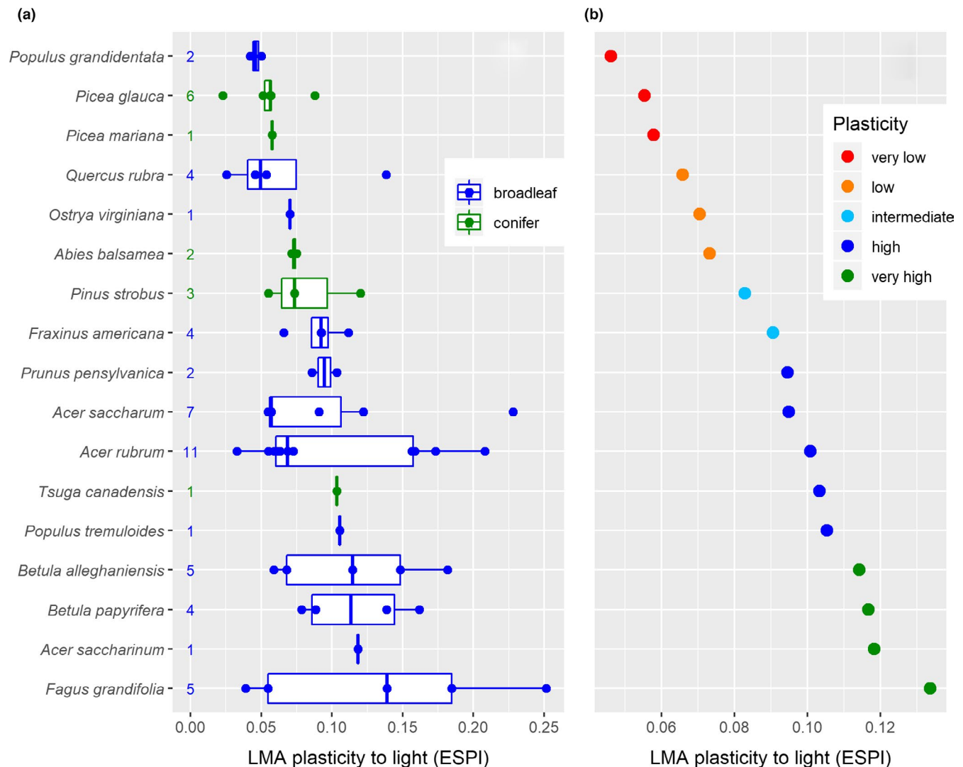
FIGURE 3 Plasticity of leaf mass per area (LMA) to light availability, calculated as the Environmentally Standardized Plasticity Index (ESPI). 17 of the 26 species were considered in this meta-analysis while no data were found in the literature for the remaining nine species (i.e., hatched cells in the “LMA plasticity to light” column in Figure 6). ESPI was calculated using the log of light availability (% of full sunlight) to account for the nonlinear relationship of LMA with light. (a) Distribution of the collected plasticity values as well as the number of observations obtained from the literature provided to the left of boxplots. (b) Average plasticity for each species. The five colors represent five groups with increasing levels of plasticity as classified using a k -means clustering. See Appendix S2 for more details on the meta-analysis
