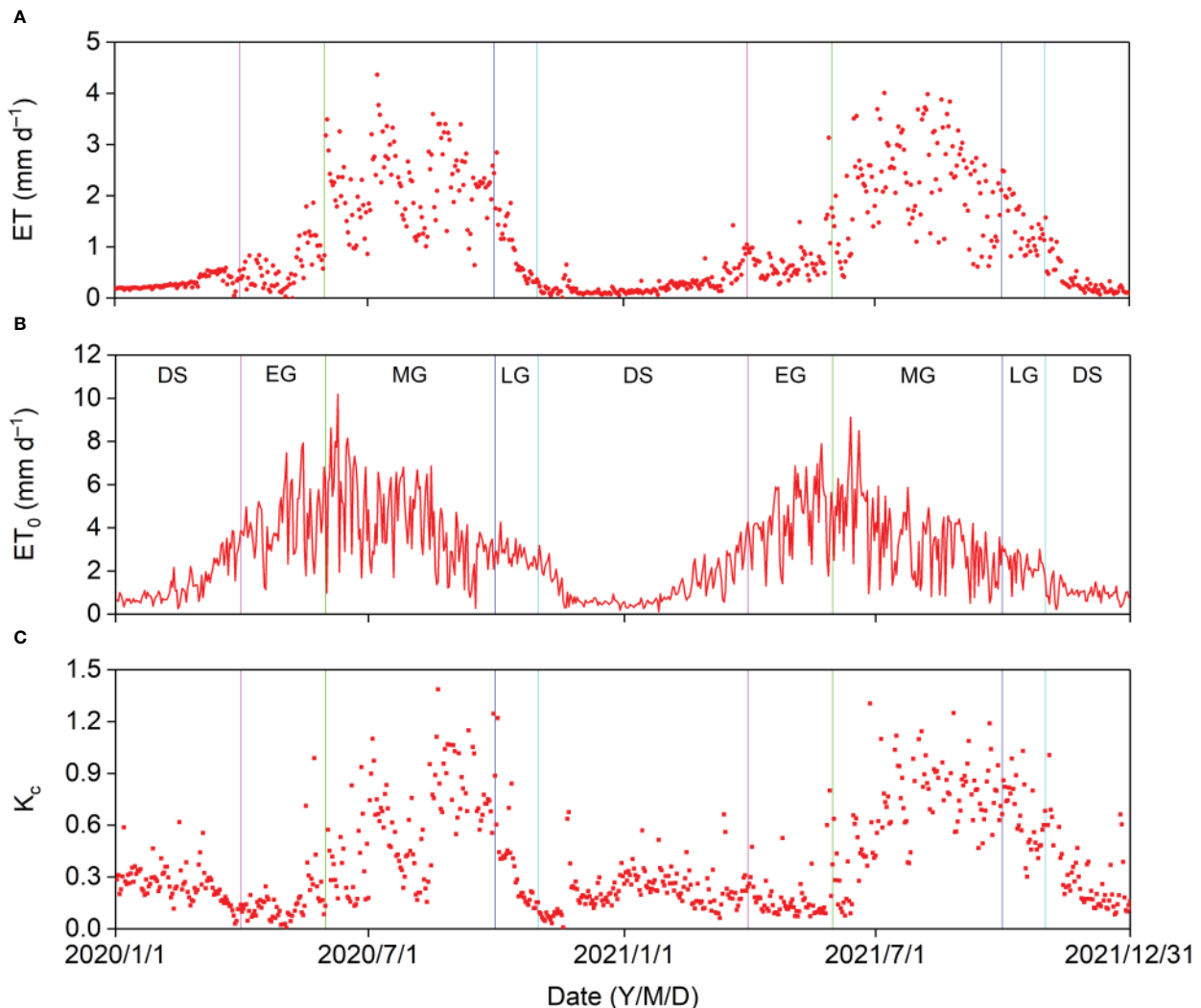
FIGURE 8 Seasonal variation in (A) evapotranspiration (ET), (B) reference evapotranspiration ( ET_0 ), and (C) crop coefficient ( K_c ) in 2020 and 2021.
