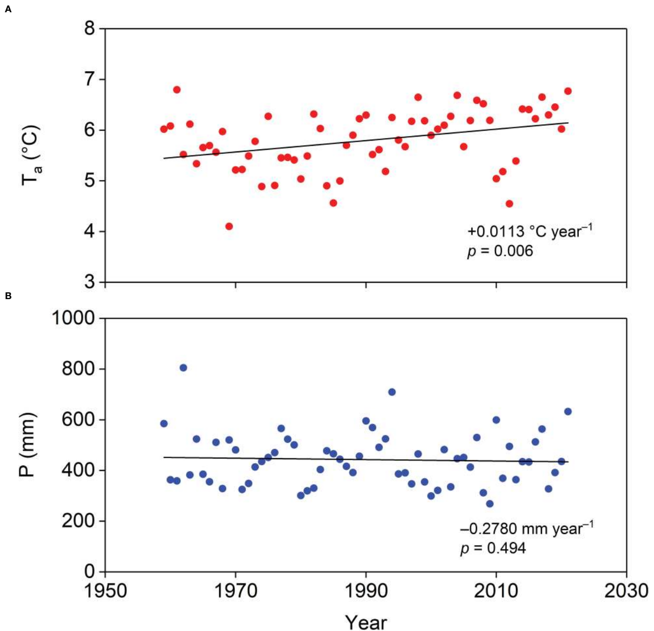
FIGURE 2 General trends in (A) annual mean air temperature ( T_a ) and (B) annual precipitation ( P ) in our study area during 1959–2021.
