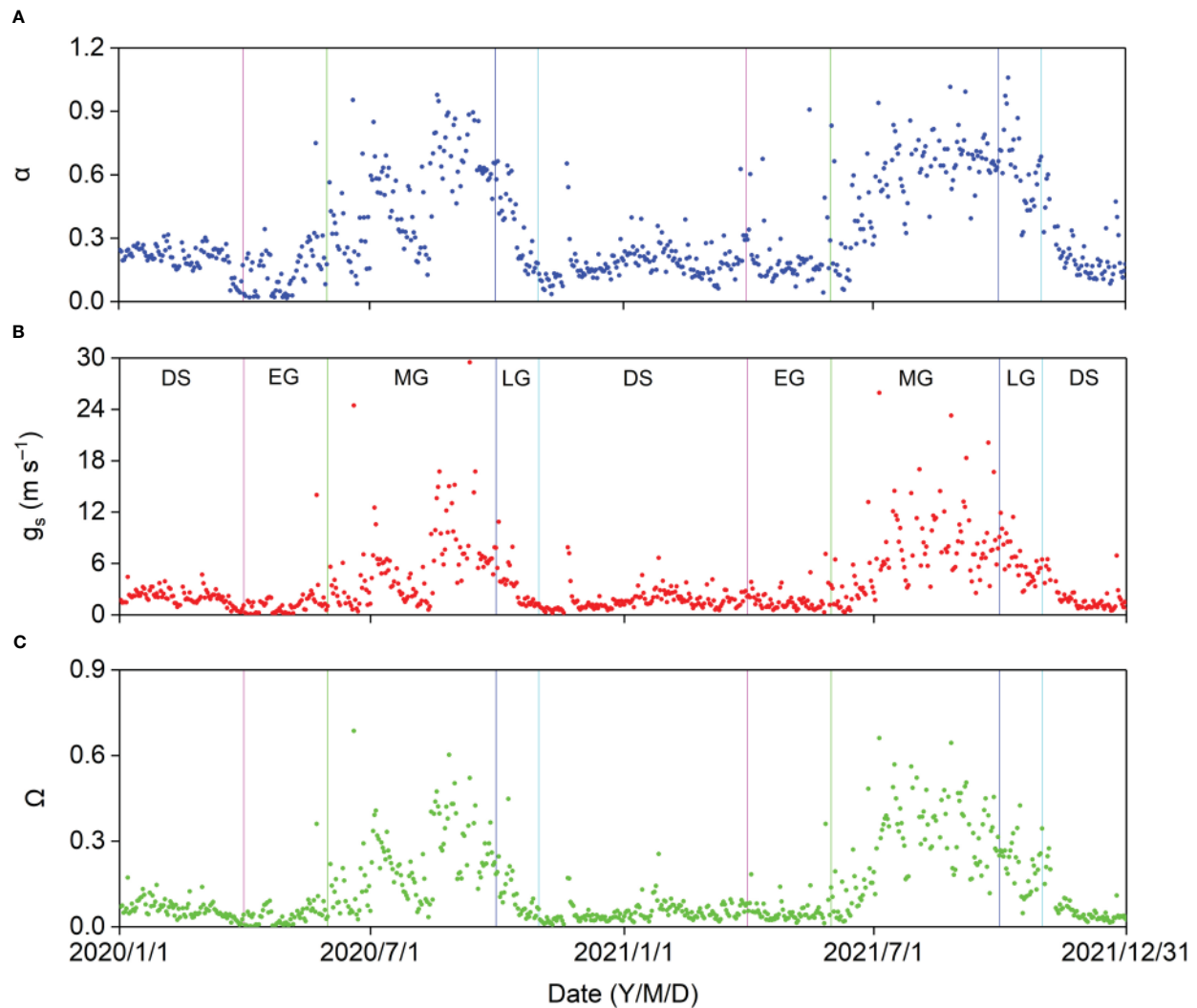
FIGURE 11 Seasonal variation in midday (A) Priestley–Taylor coefficient ( \alpha ), (B) surface conductance ( g_s ), and (C) decoupling coefficient ( \Omega ) in 2020 and 2021.
