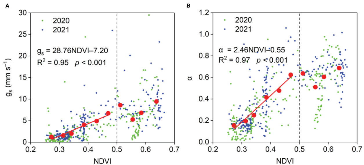
FIGURE 13 Relationships between midday (A) g_s and (B) \alpha and NDVI and during the growing season in the Pinus tabuliformis plantation. Red solid dots: the dependent variables were bin-averaged into 0.04 NDVI increments.
