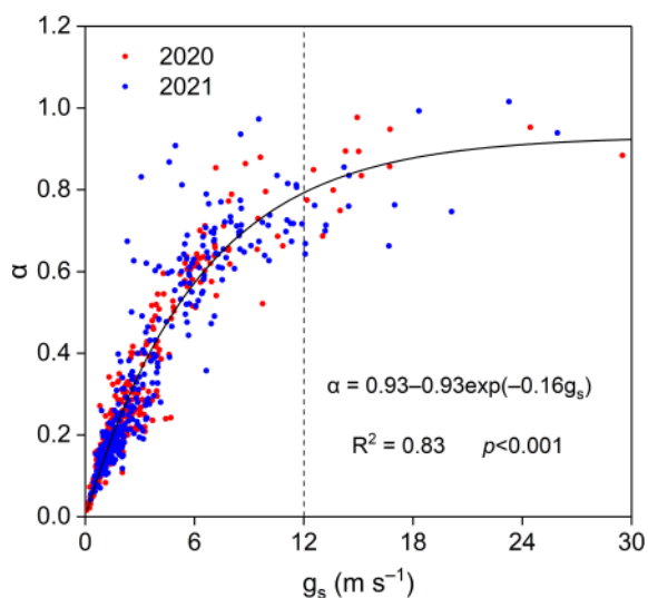
FIGURE 12 Relationship between midday \alpha and g_s in the Pinus tabuliformis plantation.
