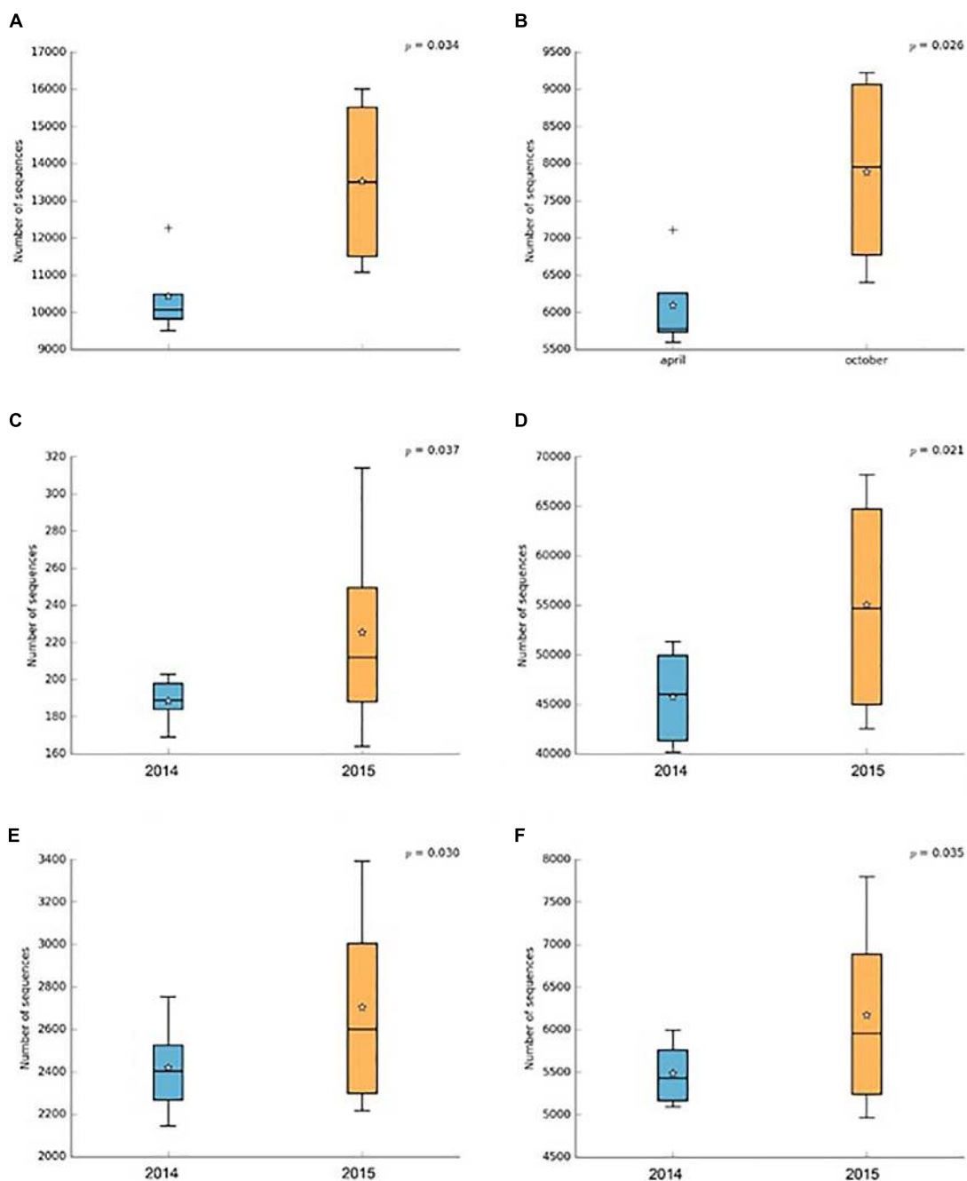
FIGURE 4 | Number of sequences assigned to genetic information [ribosome (A) and aminoacyl-tRNA biosynthesis (B)], environmental [ion channels (C) and transporters (D)] and energy metabolisms [sulfur (E) and nitrogen metabolism (F)] in the total rhizobacterial community associated with Cisthante longiscapa during full-flowering stage of 2014 and 2015 flowering desert events in Atacama Desert.
