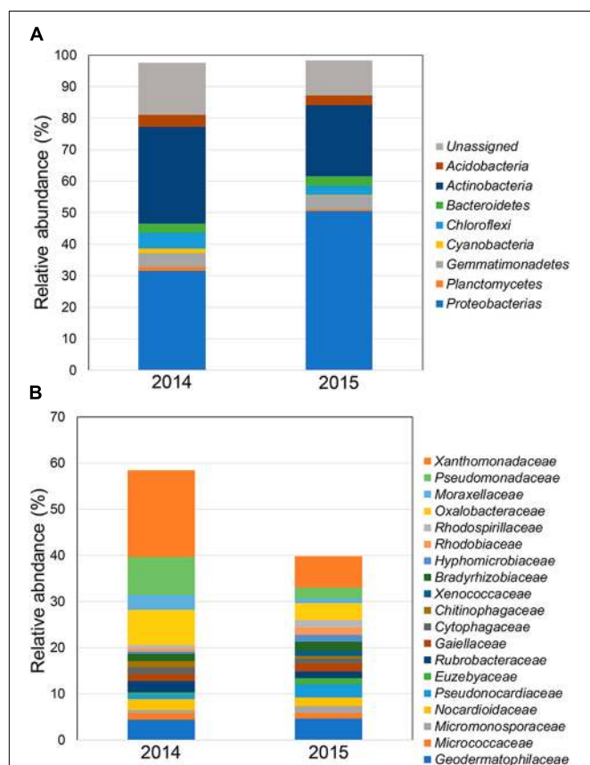
FIGURE 2 | Average of relative abundance at phylum (A) and family (B) taxonomic levels in the total rhizobacterial community associated with Cisthante longiscapa during full-flowering stage of 2014 and 2015 flowering desert events in Atacama Desert.
