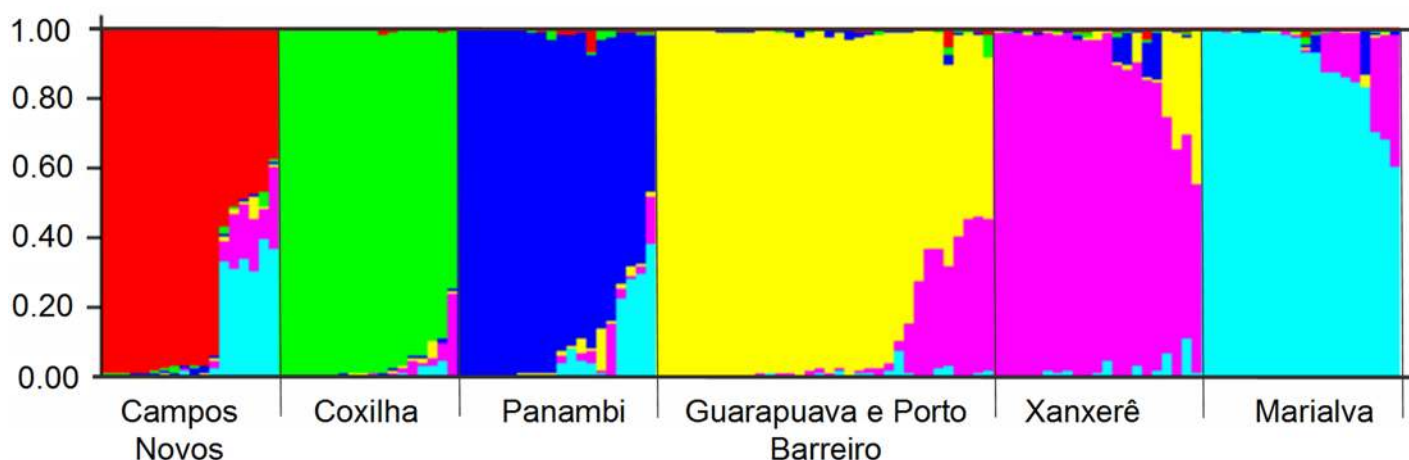
Fig 4. Genetic groups of Achyrocline flaccida (Weinm.) DC. established by Bayesian analysis using 190 ISSR loci.
