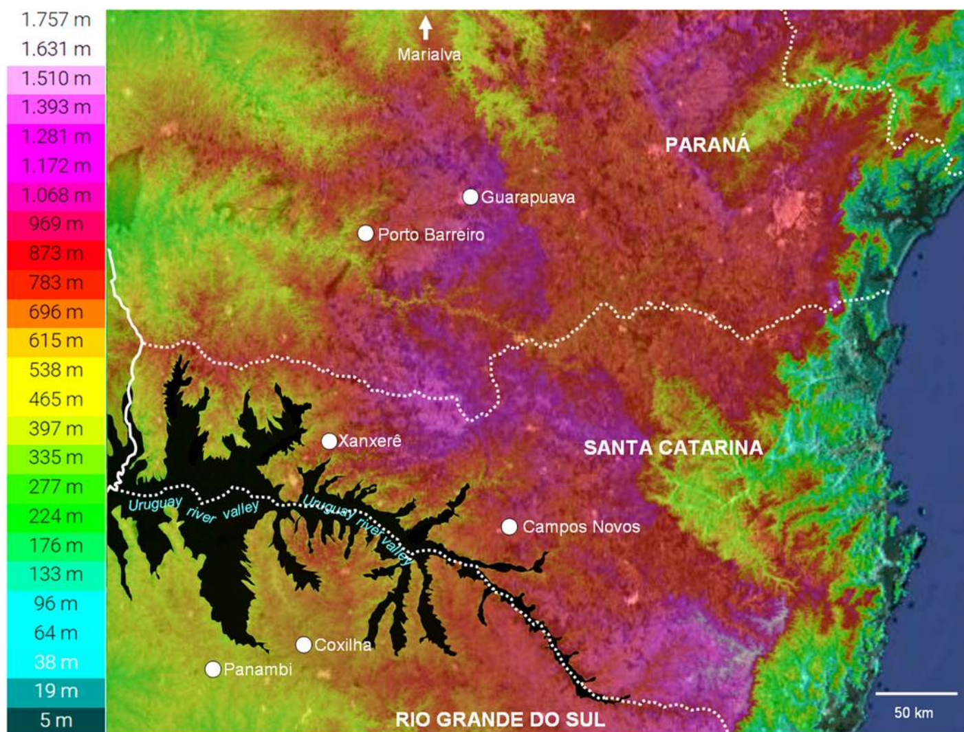
Fig 6. Topography of the southern region of Brazil. Highlight for the Uruguay River Valley (dark) and the sampling site of Achyrocline flaccida (Weinm.) DC. populations.
