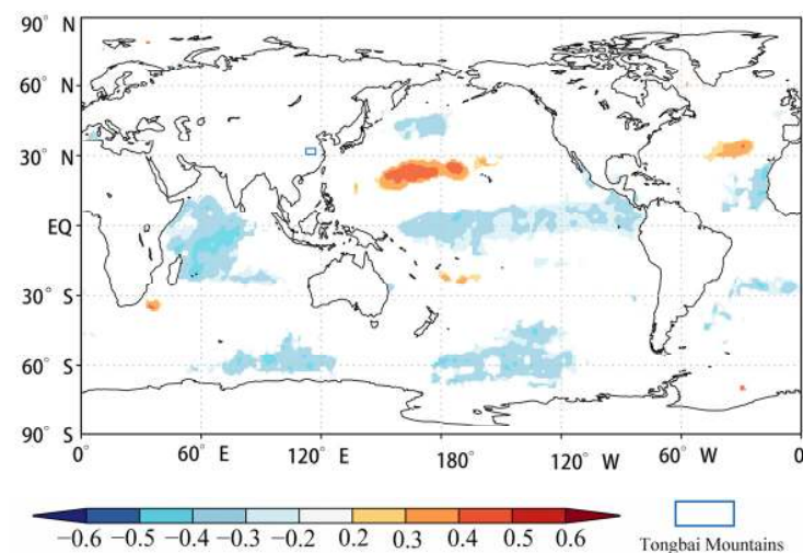
Figure 12. The spatial teleconnection between the reconstructed T_{MJ} series and the HadISST1 1° sea surface temperature during the common period of 1901–2005.
