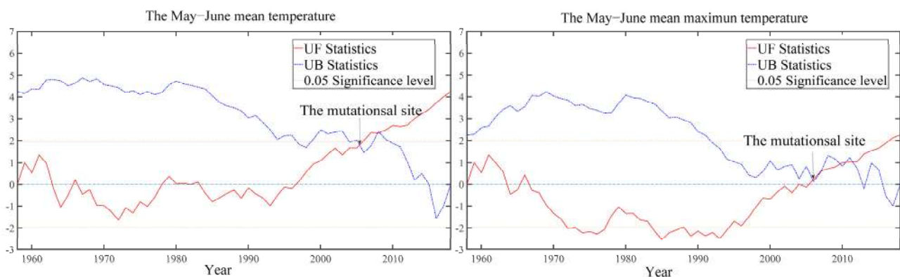
Figure 6. Mann–Kendell tests of T_{MJ} and T_{maxMJ} at the Tongbai meteorological station from 1958–2014.
