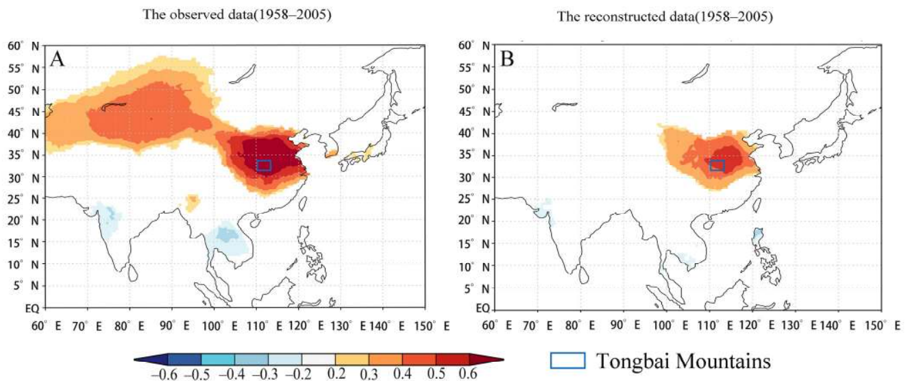
Figure 10. Spatial correlation between the observed (A) and reconstructed (B) T_{MJ} with CRU TS 4.05 ( 0.5^\circ \times 0.5^\circ ) from 1958–2005 through the KNMI climate detector, which was used in order to study the regional representativeness of the reconstructed series in China.
