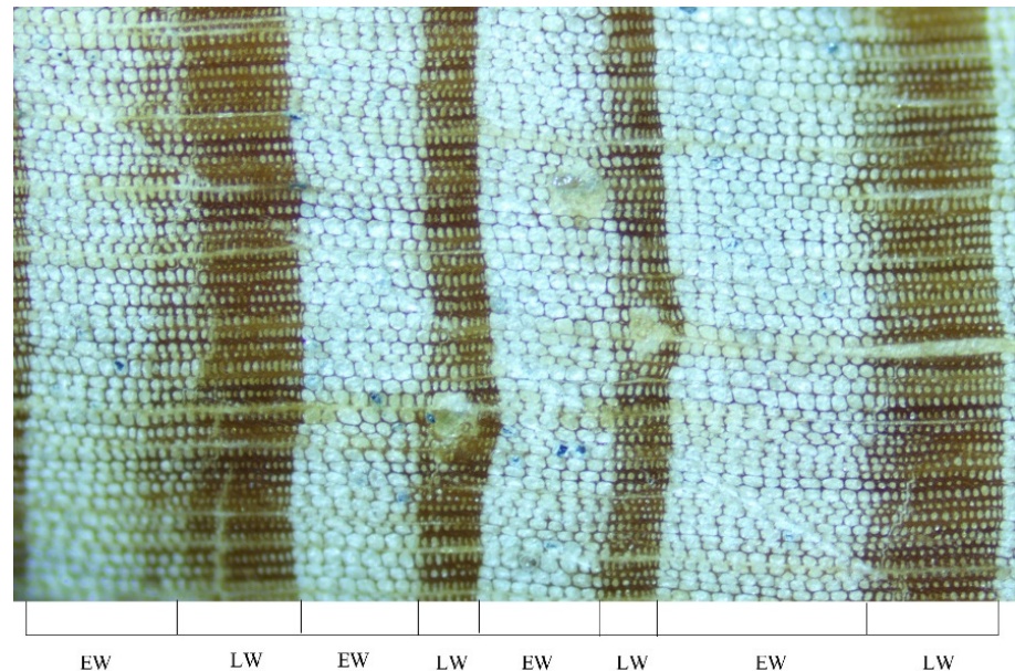
Figure 2. The boundary diagram of EW and LW of Pinus taiwanensis Hayata under a microscope, magnification of 200 times.
