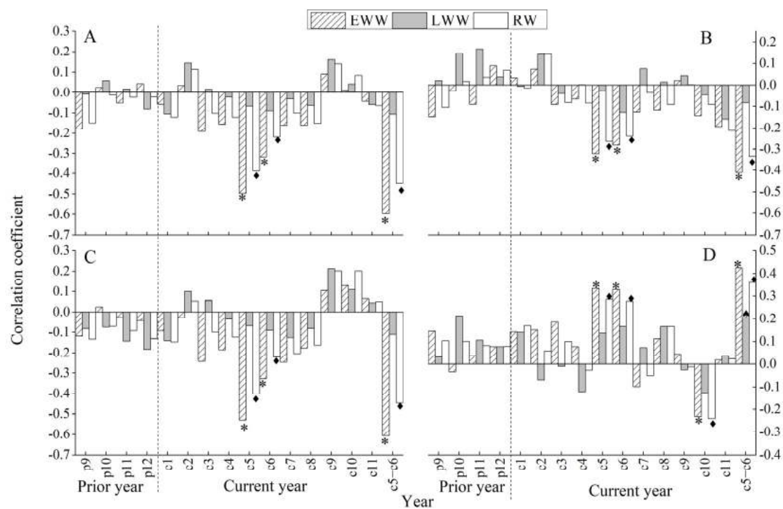
Figure 5. The correlation analyses between RES of EWW, LWW, RW and T (A), Tmin (B), Tmax (C), P (D) of the Tongbai meteorological station. *, and ♦ all stand for p < 0.05 .
