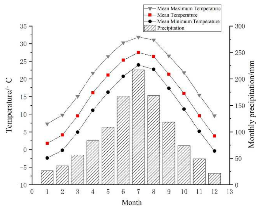
Figure 3. The distribution graph of monthly mean temperature (T), mean maximum temperature (Tmax), mean minimum temperature (Tmin) and monthly total precipitation (P) at the Tongbai meteorological station from 1958–2014.
