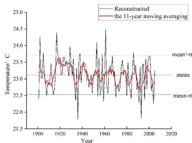
Figure 8. The reconstructed T_{MJ} curve and 11-year moving average curve in the Tongbai Mountains from 1901 to 2005.
