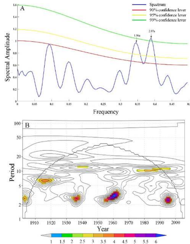
Figure 11. The periodic variation of the reconstructed T_{MJ} series from 1901 to 2005 in the Tongbai Mountains using the power spectrum analysis (A) and wavelet analysis (B); 2.07a and 1.96a (A) are significant cycles of the reconstructed T_{MJ} from 1901 to 2005 in the Tongbai Mountains, which reach 99% and 95% confidence levels, respectively.
