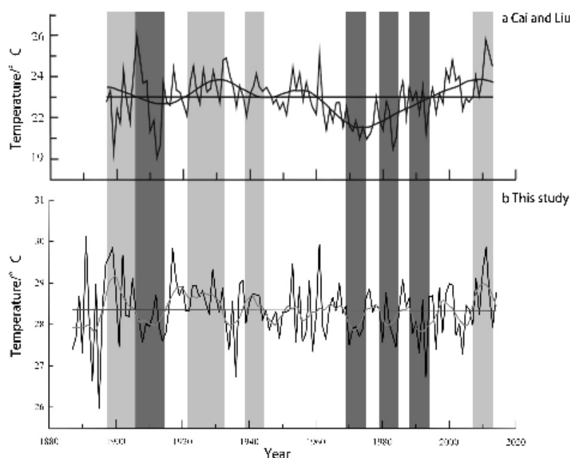
Figure 9. The comparison of the moving average curves of the reconstructed T_{MJ} in this study (b) and the reconstructed May–July mean minimum temperature of Cai and Liu (a) in the Tongbai Mountains. Dark colors and light colors represent warm periods and cold periods, respectively.
