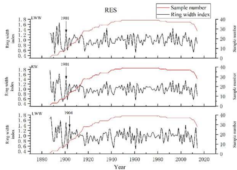
Figure 4. RES of EWW, LWW and RW and the samples of Pinus taiwanensis Hayata in the Tongbai Mountains. (Arrow shows the beginning year of SSS > 0.85).
