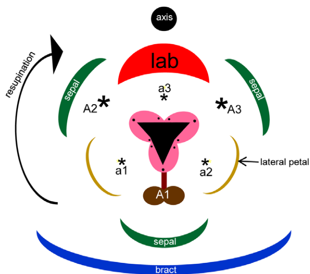
Figure 1 Floral diagram of Herminium monorchis , typical of orchidoid orchids. Asterisks indicate expected locations of missing stamens, based on comparison with a typical trimerous–pentacyclic monocot flower (e.g. Rudall & Bateman, 2002). Abbreviations: a = inner-whorl stamens, A = outer-whorl stamens, lab = labellum.
