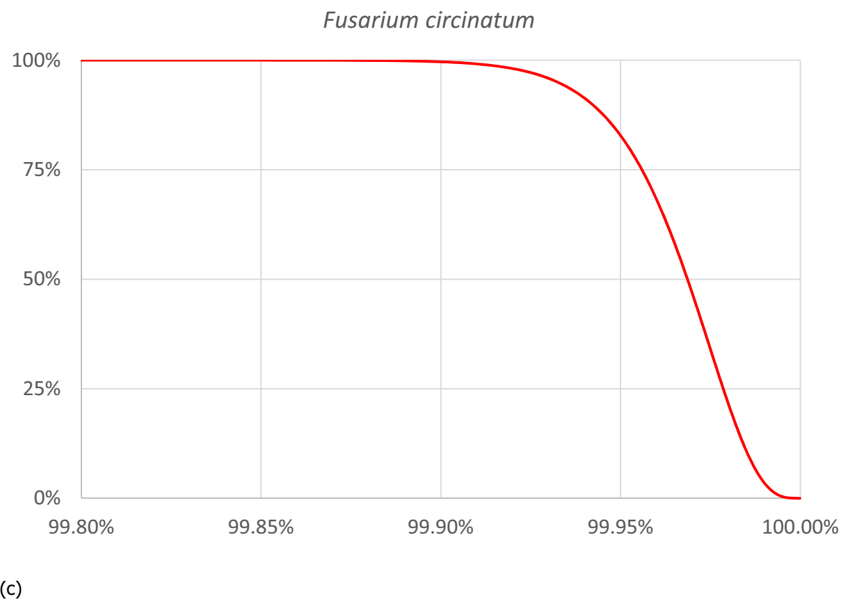
Figure B.5: (a) Comparison of judged values for the uncertainty distribution of pest infestation per 10,000 bonsai plants (histogram in blue) and fitted distribution (red line); (b) density function to describe the uncertainties of the likelihood of pest freedom; (c) descending distribution function of the likelihood of pest freedom
