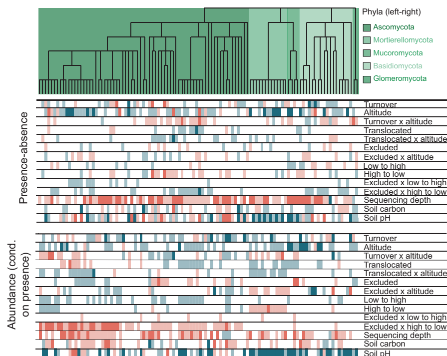
FIGURE 2 Fungal species-level responses to each predictor, both for presence-absence and abundance conditional on presence fungal models. The darker red blocks indicate a positive response of fungal species with \geq 95\% posterior probability, and the darker blue blocks indicate a negative response with \geq 95\% posterior probability. The lighter blue and red blocks indicate a response with \geq 75\% posterior probability. See Table S3 for a list of the fungal species.
