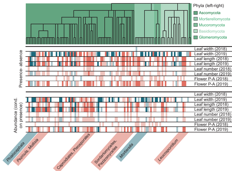
FIGURE 4 Associations between fungal presence-absence and abundance and plant growth traits in the 'fungal-plant model'. The darker red blocks indicate a positive response of fungal species with \geq 95\% posterior probability, and the darker blue blocks indicate a negative response with \geq 95\% posterior probability. The lighter blue and red blocks indicate a response with \geq 75\% posterior probability. See Table S3 for a list of the fungal species.
