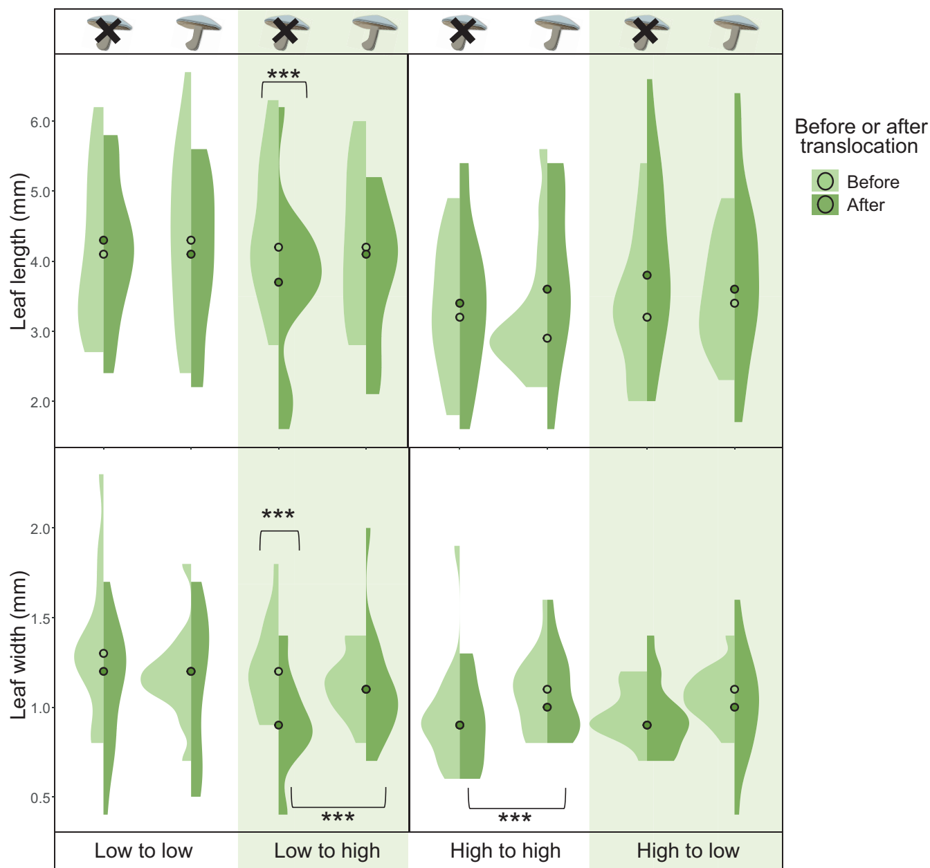
FIGURE 3 Bistorta vivipara leaf width and length for each treatment before and after translocation, with statistical support (***) based on \geq 95\% posterior probability. Numerical values of the posterior probabilities are given in Table S9.
