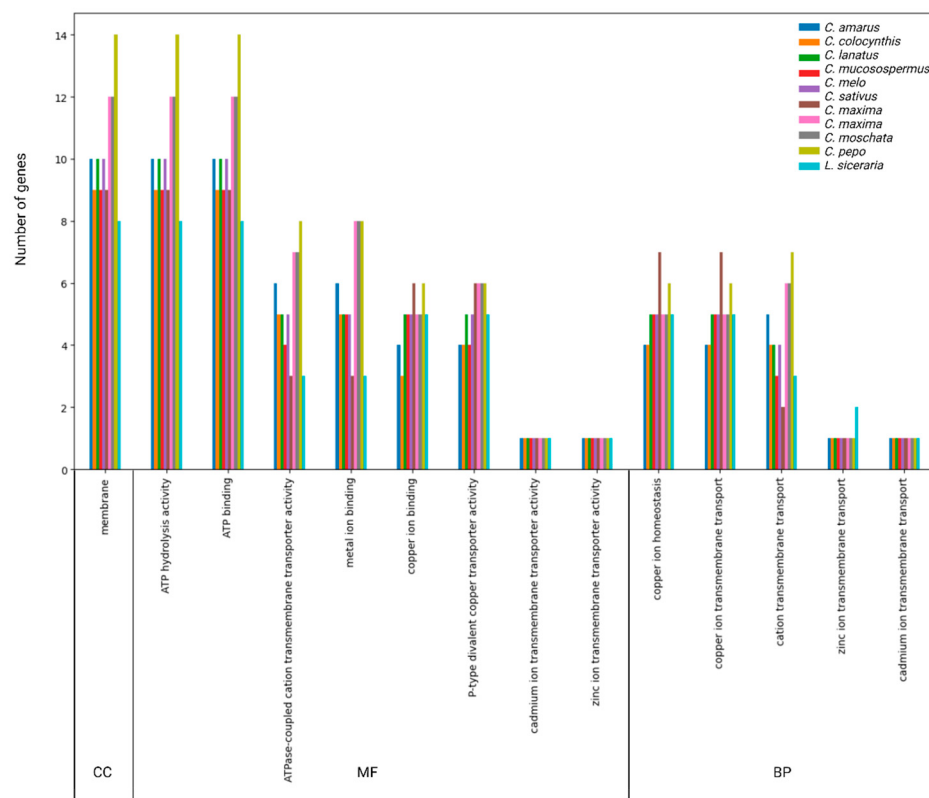
Figure 6. Gene ontology analysis results for Cucurbit species. Cellular Component (CC), Molecular Function (MF), and Biological Processes (BP) were identified with the OmicsBox program. Specific results for genes of each species are found in Supplementary Table S5.
