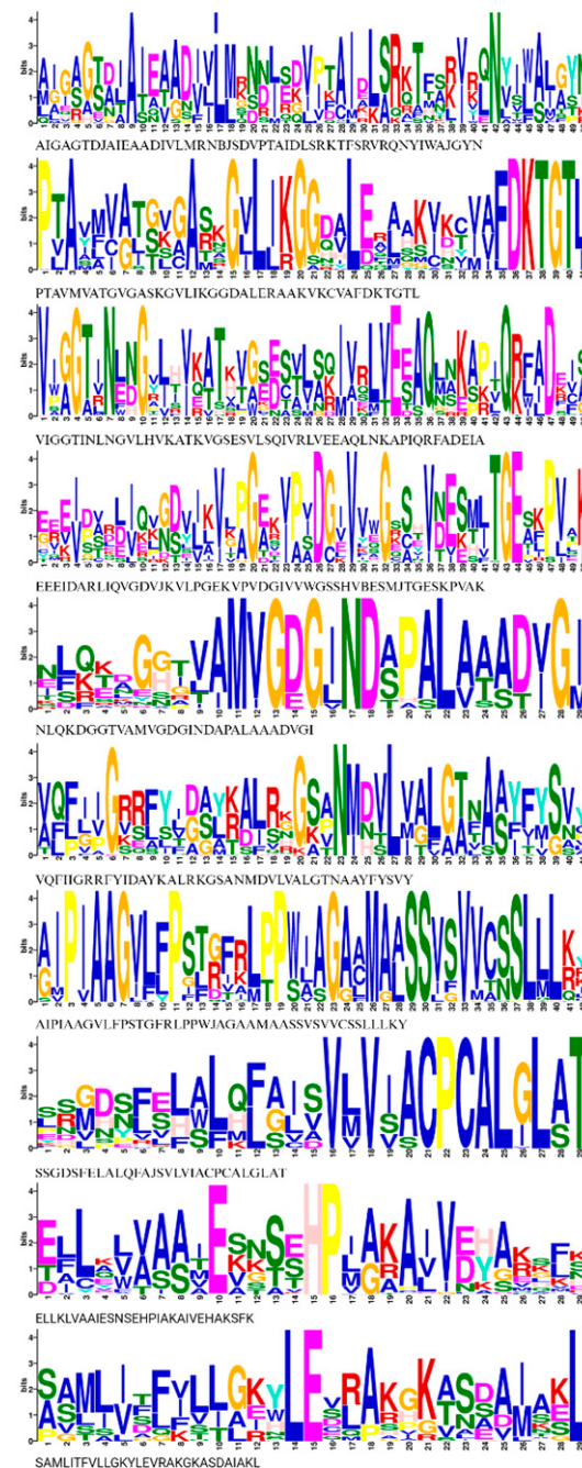
Figure 5. Common conserved motifs of HMA proteins among Cucurbitaceae plants: C. amarus , C. colocynthis , C. lanatus , C. mucospermus , C. melo , C. sativus , C. maxima , C. moschata , C. pepo , and L. siceraria . The overall height of the stack indicates the degree of sequence conservation. The height of residues suggests the relative frequency of each residue at that position. Typed sequences of motifs are represented below each stack.
