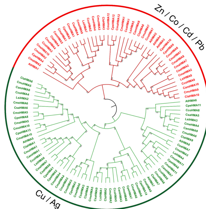
Figure 3. Phylogenetic relationship of the HMA gene family. Phylogenetic analysis of Cucurbits and Arabidopsis was carried out using the neighbor-joining method with 1000 bootstraps. Based on genetic and functional studies, the phylogeny was divided into two major clades, P1B-ATPases; zinc (Zn)/cobalt (Co)/cadmium (Cd)/lead (Pb) group is highlighted in red, and the copper (Cu)/silver (Ag) group is highlighted in green.
