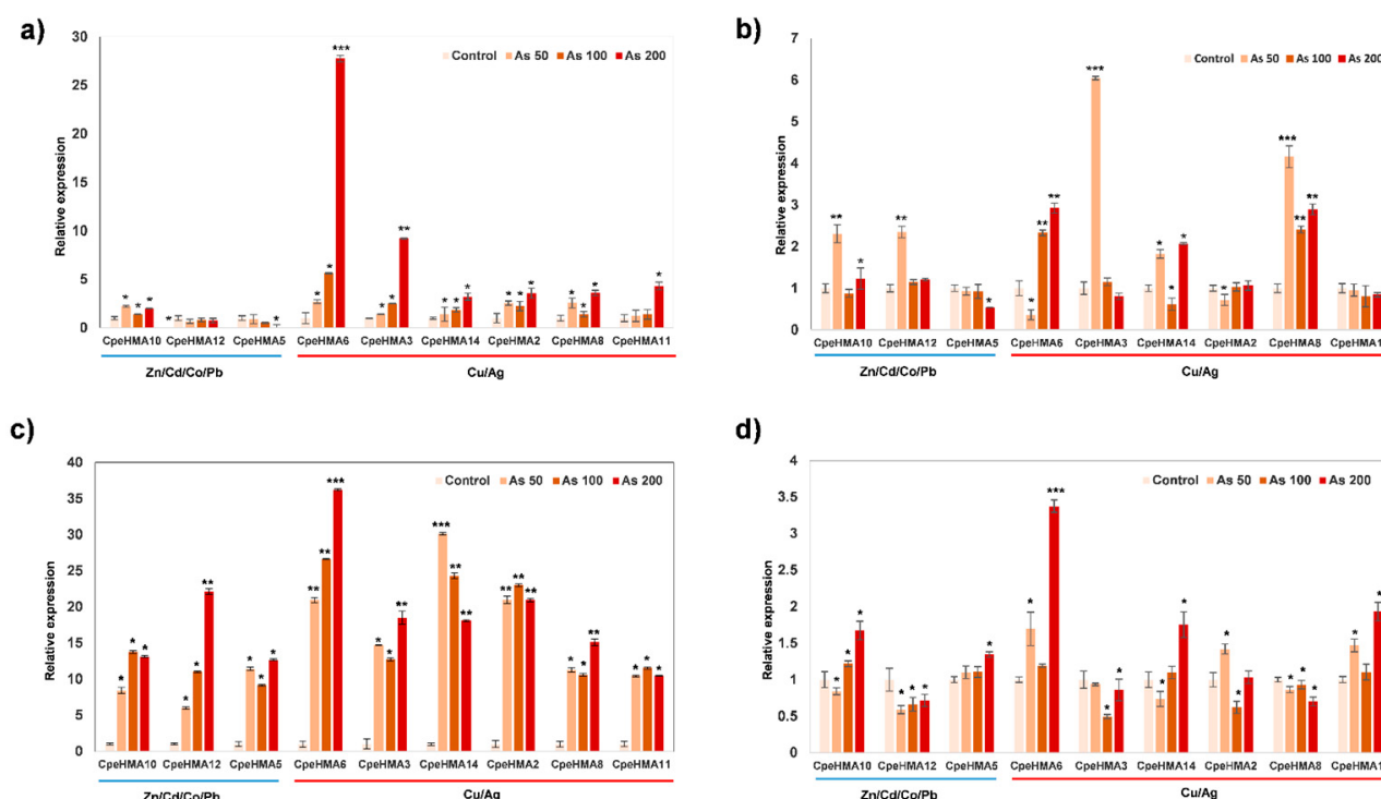
Figure 8. Expression pattern of HMA genes from C. pepo in different tissues under As stress. Relative expression levels of the CpHMA genes in (a) root, (b) leaf, (c) flower, and (d) fruit tissue of C. pepo plants treated with 50, 100, and 200 \mu M of arsenic in soil were determined with qRT-PCR. The gene expression level for each HMA gene in the control plants with no As was normalized to 1, as the 2^{-\Delta\Delta CT} method suggests. The results represent the means of the biological replicates with their standard deviation represented as error bars. “*”, “**”, and “***” indicate genes statistically significantly differentially expressed between the treatment and the control using a t -test at the level of p \leq 0.05 , p \leq 0.01 , and p \leq 0.001 , respectively.
