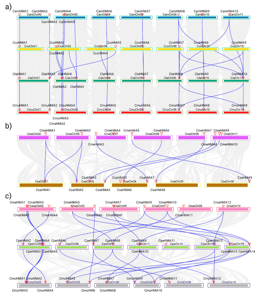
Figure 4. Collinearity analysis between the HMA gene family in Cucurbitaceae species. (a) Synteny between the Citrullus genera: C. amarus (dark blue), C. colocynthis (yellow), C. lanatus (dark green), and C. mucospermus (red). (b) Synteny between the Cucumis genera: C. melo (purple) and C. sativus (brown). (c) Synteny between the Cucurbita genera: C. maxima (pink), C. pepo (light green), and C. moschata (gray). The collinearity analysis was visualized using TBTools with an E-value < 1 \times 10^{-10} .
