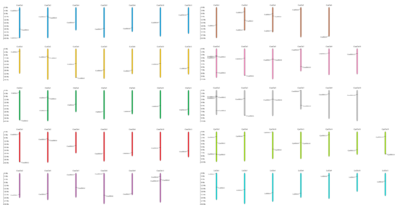
Figure 1. Chromosomal locations of HMA genes in C. amaratus (dark blue), C. colocynthis (yellow), C. lanatus (dark green), C. mucospermus (red), C. melo (purple), C. sativus (brown), C. maxima (pink), C. moschata (gray), C. pepo (light green), and L. siceraria (light blue). Chromosome numbers are represented at the top of each chromosome. The left panel scale indicates the chromosome length in Mb.
