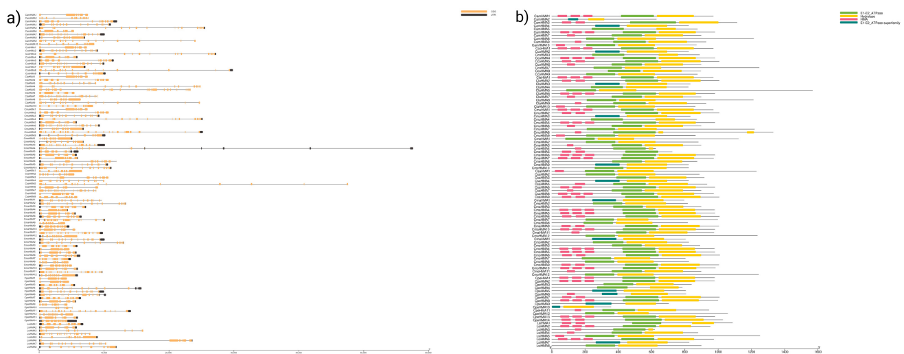
Figure 2. Gene structure and protein domains of the HMA family in Cucurbit species. (a) Exon/intron structures of HMA genes. Exons are represented as orange boxes, introns as strings, and promoter UTRs in black. (b) The protein domain structure pattern of HMA gene family, and different-colored rectangles represent different structural domains; the green rectangles represent E1-E2 ATPase; the yellow rectangle represents hydrolase; the pink rectangle represents HMA; the dark-green rectangle represents E1-E2 ATPase superfamily. The gene name is on the left side of each sequence, and the below scale indicates the length in kb and aa, respectively.
