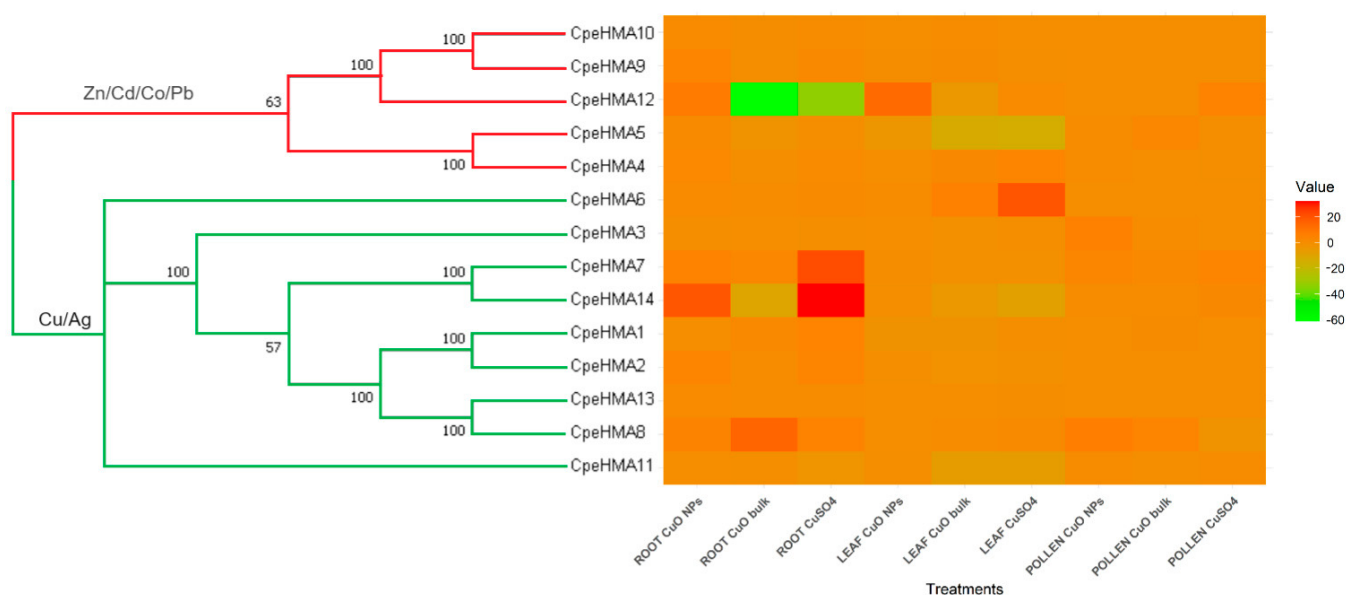
Figure 7. Phylogenetic tree and heat map of gene expression levels of HMA genes in root, leaf, and pollen tissues of C. pepo exposed to CuO NPs, bulk CuO, and bulk CuSO 4 (Accession: GSE173716). The bar to the right of the heat map represents normalized expression values in each treatment.
