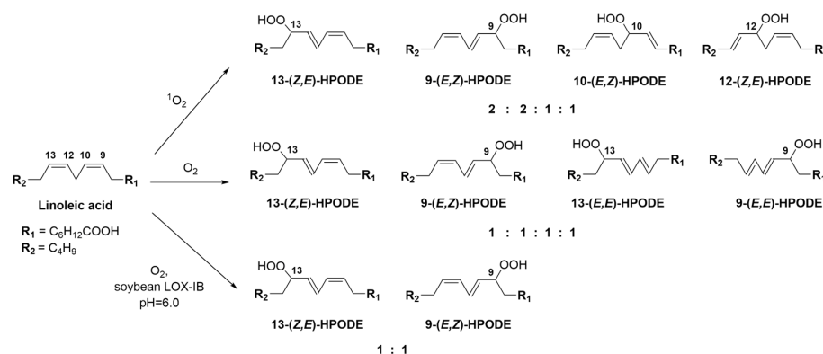
Scheme 1. Isomers of hydroperoxyoctadecadienoic acid (HPODE) formed during oxidation of linoleic acid. Different products are formed during oxidation by singlet oxygen ( ^1O_2 ), atmospheric oxygen ( O_2 ) and soybean lipoxygenase (LOX-IB), shown with relative ratio of products [15].
