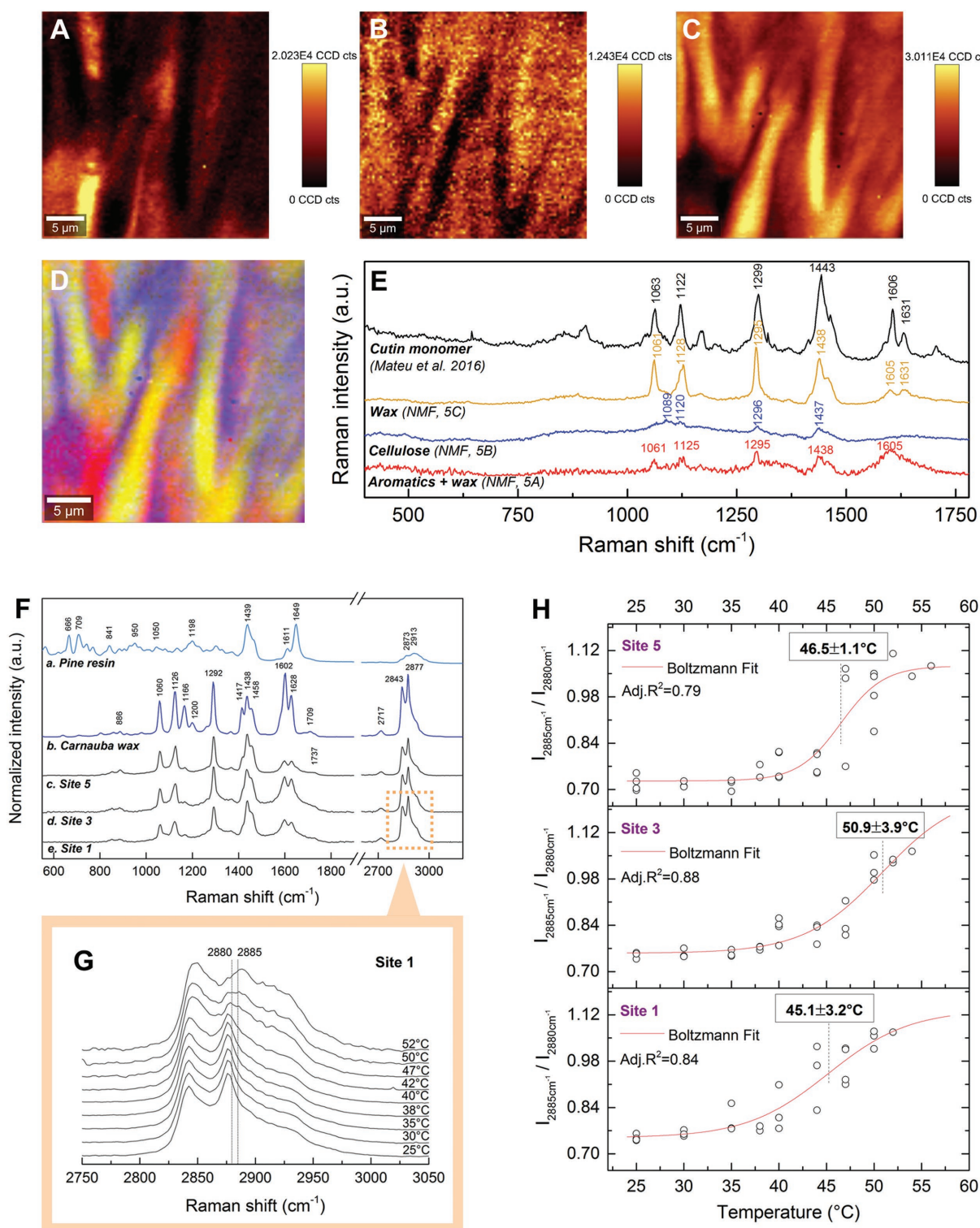
Figure 5. Physicochemical analysis of the junction zone. Chemical mapping (in situ Raman images obtained via non-negative matrix factorization (NMF) analysis) of an area in the JZ (site 1, box in Figure 4B); indicating the presence of A) aromatic compounds/wax along with B) cellulose in the interdigitating tooth-like structures and C) waxes (cutin) in between. D) Overlay of (A) (red), (B) (blue), and (C) (yellow). E) Spectra of cutin and the compounds in the JZ obtained via NMF. F) Raman spectra of two reference standards ( P. banksiana resin and Carnauba wax) and of the JZs of B. attenuata follicles from three different sampling sites (all are in situ measurements at room temperature). Nonindicated peak positions in spectra (c–e) correspond to the ones in (b). G) Spectral features of the C–H stretching region at different temperatures. Relevant band positions are indicated. H) Melting behavior of the waxes present in the JZs of follicles from sites 5, 3, and 1 (inflection points indicated with \pm SE). Data points represent the intensity ratio of the band at 2885\text{ cm}^{-1} relative to the one at 2880\text{ cm}^{-1} .
