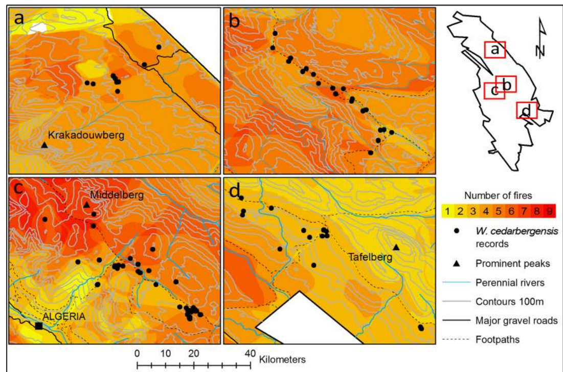
Fig. 4 Fire frequency map for the four studied regions within the Cederberg Wilderness Area. a Heuningvlei, b Skerpioenspoort, c Middelberg and d Welbedacht. The fire record is from 1944 to 2012
