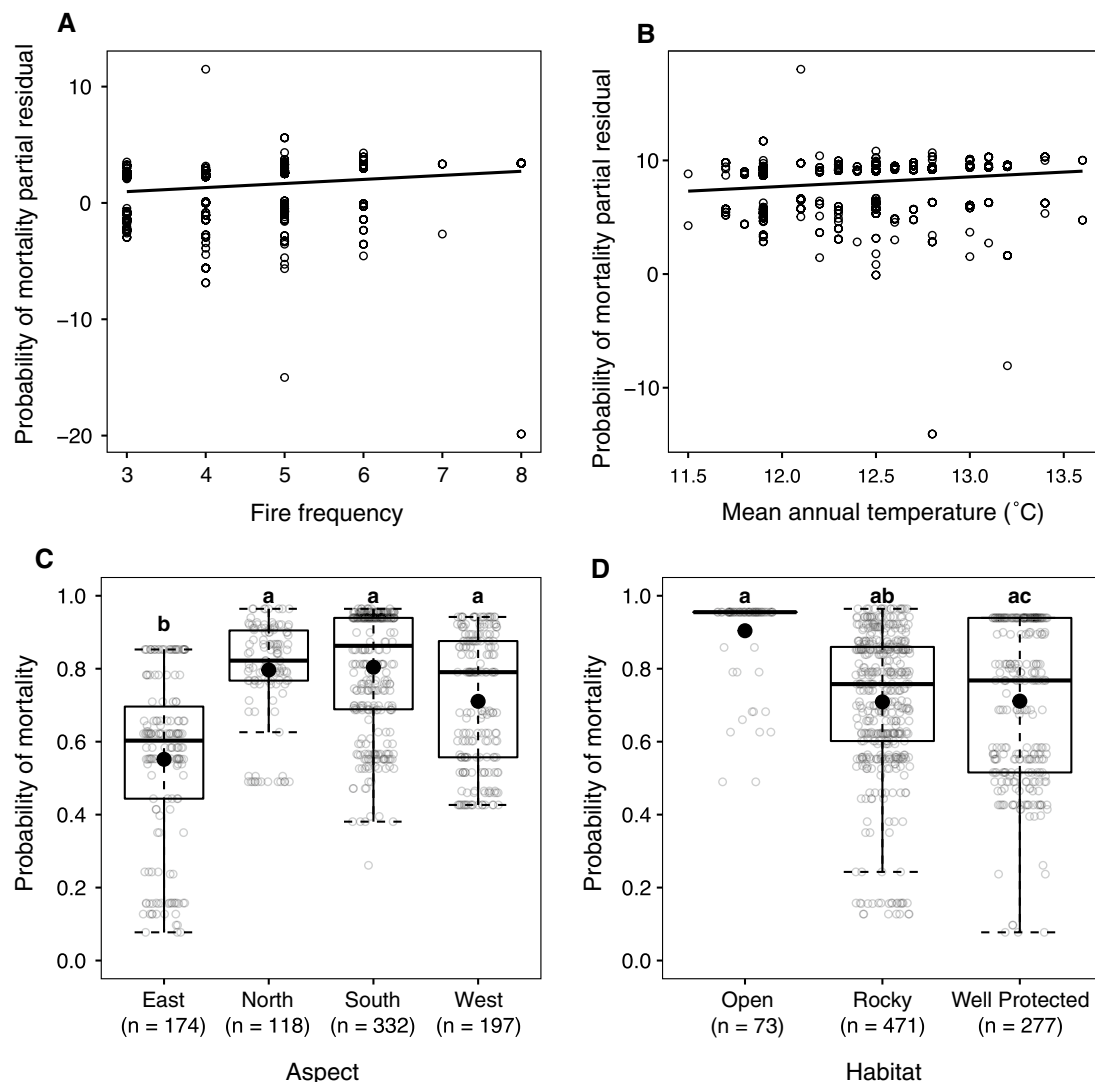
Fig. 6 A–D Partial residual plots ( A, B ) and predicted points ( C, D ) showing the probability of Widdringtonia cedarbergensis mortality (Model 3) only natural populations in relation to environmental and climatic variables. Regression lines indicate the partial fit for A fire frequency and B mean annual temperature; and raw predicted with Tukey boxplots for C aspect and D habitat indicate the median, lower and upper quartiles, and minimum and maximum values with outliers outside the whiskers. Means are shown as filled black dots. Different letters indicate where the modelled probability of mortality was significantly different between aspects or habitat ( p < 0.05 )
