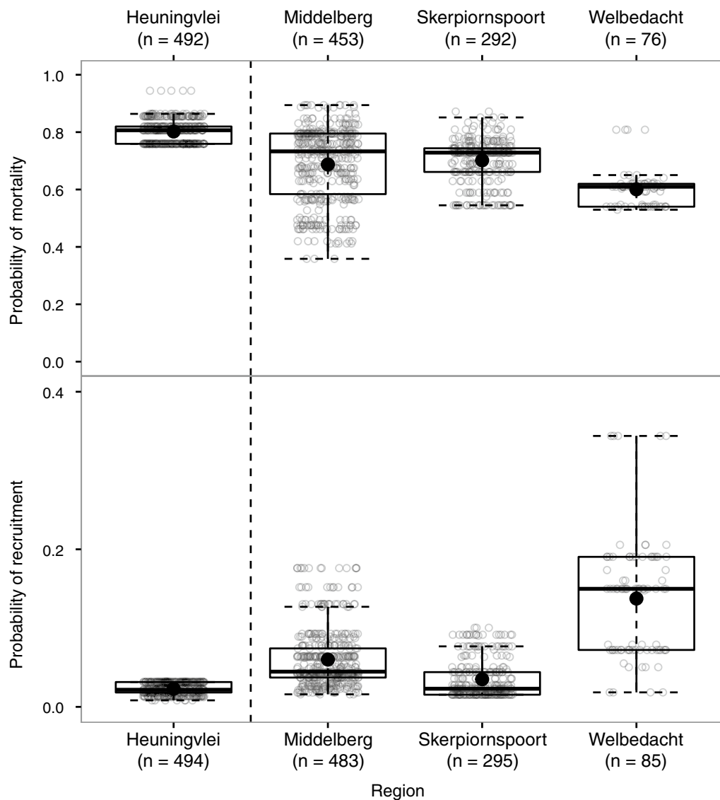
Fig. 3 Modelled probability of Widdringtonia cedarbergensis mortality (Model 1) and recruitment (Model 2) at all sampled regions. Raw predicted points with Tukey boxplots indicating the median, lower and upper quartiles, and minimum and maximum values with outliers outside the whiskers. Means are shown as filled black dots
