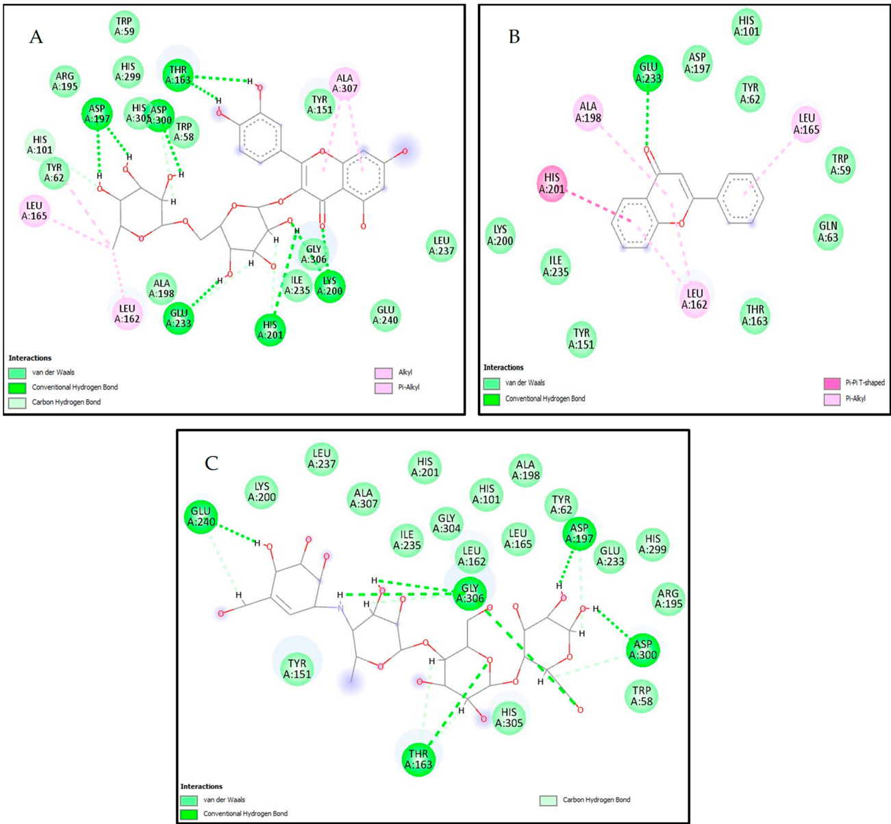
Figure 1. 2D intermolecular interactions between (A) rutin, (B) flavone, and (C) acarbose (standard) with the active site of \alpha -Amylase (PDB: 1B2Y) protein.
