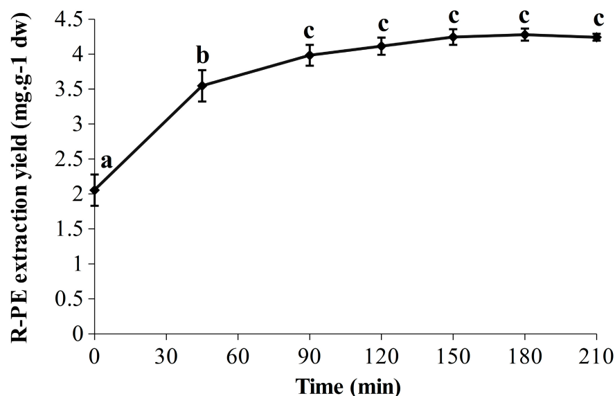
Figure 2. Evolution of the R-PE extraction yield (210 min) in optimized conditions of ultrasound-assisted enzymatic hydrolysis (UAEH) (300 W, 20 °C, 145 L·h -1 ). Values are means \pm SD from three independent experiments ( n = 3 ). Significant differences ( p < 0.05 ) are indicated by different letters.
