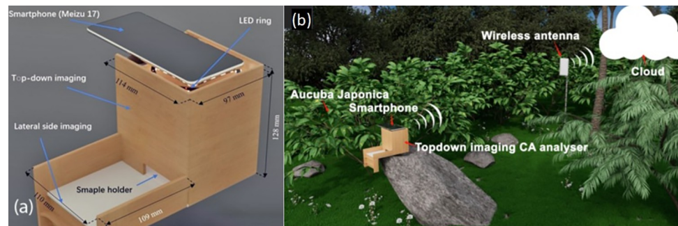
Fig 2. (a) 3D model of custom attachment. Top-down imaging occurs at the top using a white light-emitting diode (LED) ring to uniformly illuminate the drop evenly from the top. (b) contact angle analyser in a simple schematic of an ecosystem with plants used in this work.
