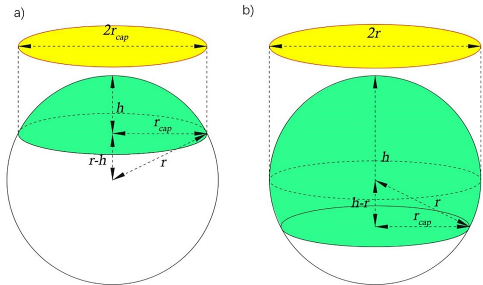
Fig 3. Schematic drawing of top-down imaging drop dimensions for a) hydrophilic and b) hydrophobic surfaces.
