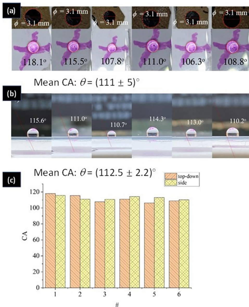
Fig 5. a) Contact angle, CA, measured by the top-down analysis; b) CA measured by side-view analysis using a tangential fit. The mean and standard deviation is shown below the figures a) and b); c) plot of CA versus # corresponding to the sequence of the measured drops in a) and b).
