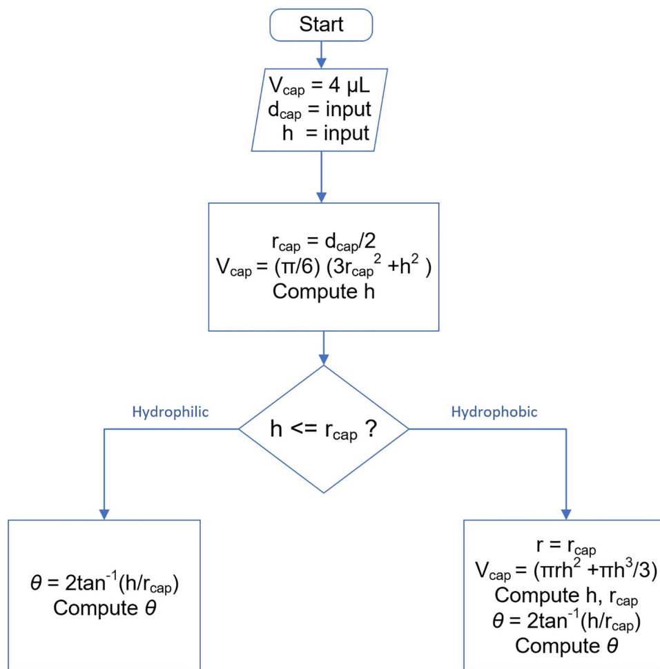
Fig 4. Flow diagram showing the decision-making process to distinguish between hydrophilic and hydrophobic cases.
