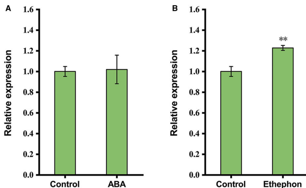
Figure 7 Expression of HdSTM under phytohormone treatments. A, Expression of HdSTM under 100 \mu M ABA treatment. B, Expression of HdSTM under 100- \mu M ethephon treatment. Error bars represent \pm SD (n = 3). Asterisks indicate significant difference relative to control (Student's t test: ** P < 0.01).
