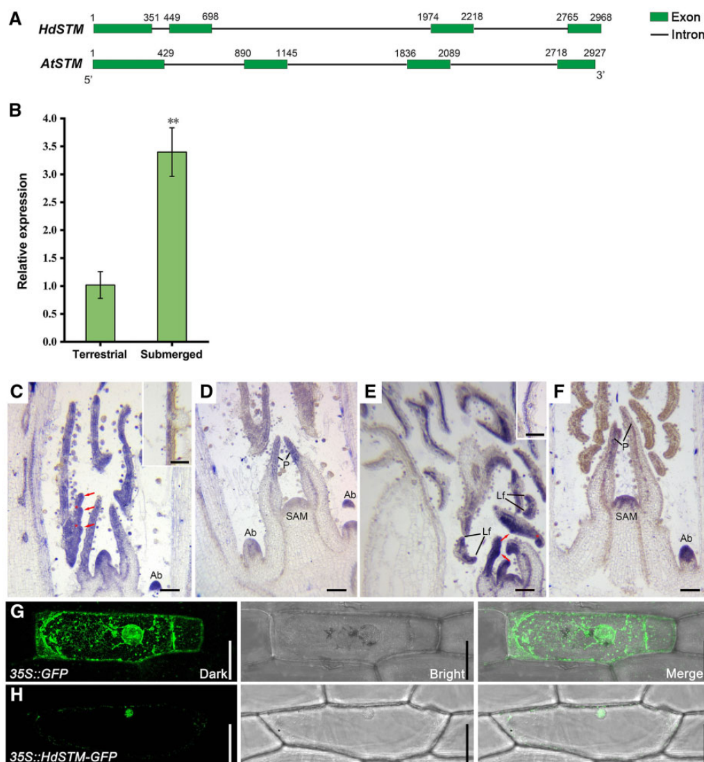
Figure 2 Expression analysis and subcellular localization of HdSTM . A , Gene structures of HdSTM and AtSTM . Both HdSTM and AtSTM contain four exons and three introns. Green boxes represent exons, and black lines represent introns. Numbers represent the positions of exon sequences. B , Expression of HdSTM in the shoot of H. difformis under terrestrial or submerged conditions. Error bars represent \pm SD ( n = 3 ). Asterisks indicate a significant difference relative to terrestrial shoot (Student's t test: ** P < 0.01 ). C , RNA in situ hybridization of HdSTM in a terrestrial shoot. Note that expression of HdSTM can be detected in the serration (arrows) and boundary (stars) of terrestrial leaves. D , RNA in situ hybridization of HdSTM in SAM and leaf primordia from a terrestrial shoot apex. E , RNA in situ hybridization of HdSTM in a submerged shoot. Note that expression of HdSTM can be detected in the emerging leaflet (arrows) and boundary (star) of submerged leaves. F , RNA in situ hybridization of HdSTM in SAM and leaf primordia from a submerged shoot apex. Local images in ( C ) and ( E ) showed the adaxial location of HdSTM in developing leaves. P, primordia; Lf, leaflet primordia; Ab, axillary buds. G and H , Subcellular localization performed in onion showed that HdSTM mainly localized to the nucleus. GFP driven by the 35S promoter was used as a control. GFP is shown in green. The left, middle, and right panels show darkfield, brightfield, and merged images. Bars = 0.5 mm in ( C – F ). Bar = 50 \mu m in ( G and H ).
