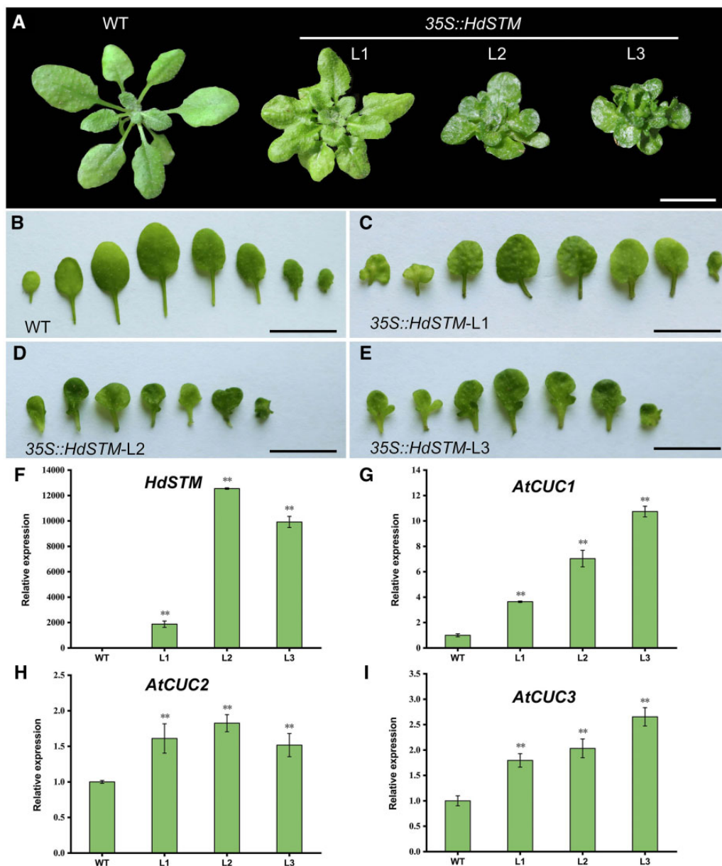
Figure 3 Heterologous ectopic expression of HdSTM in A. thaliana . A–E, Phenotypes of whole plants (A) and leaves (B–E) of WT and 35S::HdSTM transgenic plants. Images in (A) were digitally extracted from original pictures for comparison. Note that 35S::HdSTM rosette leaves developed shorter petioles and lobed leaf margins than the WT's shallow, serrated leaves. F–I, Expression analysis of HdSTM and AtCUCs in WT and transgenic plants by RT–qPCR. Error bars represent \pm SD ( n = 3 ). Asterisks indicate a significant difference relative to WT (Dunnett's test: ** P < 0.01 ). Bars = 1 cm in (A–E).
