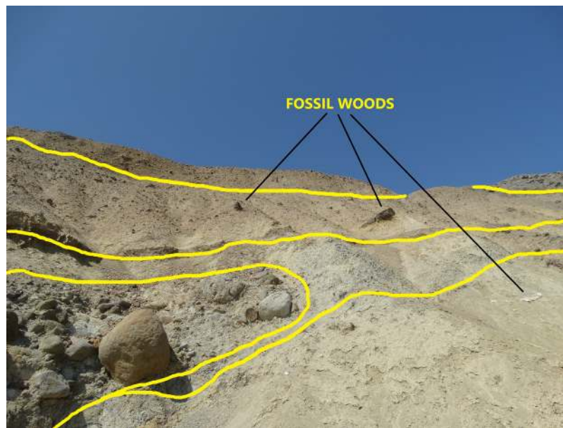
Figure 3 The outcrop of the plant fossiliferous locality in Gökçeada, showing fossil woods of different fossilization types occurring in different depositional units.
