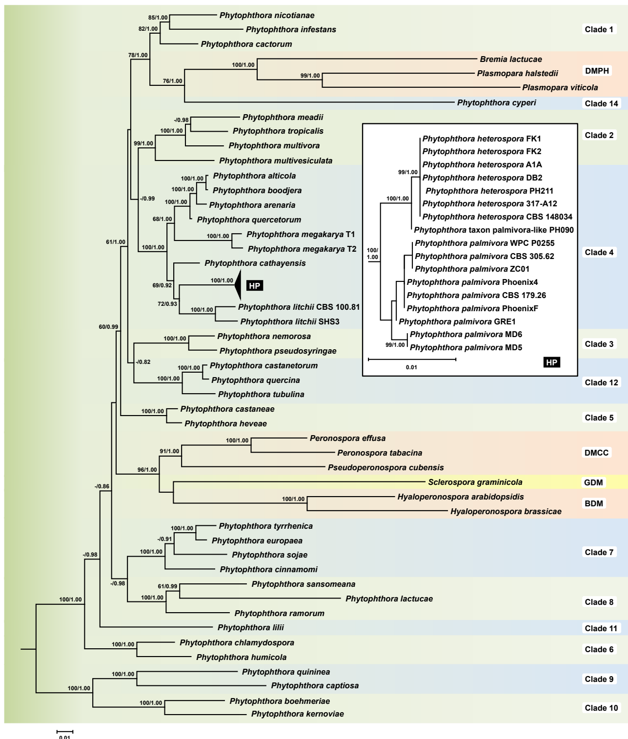
Figure 2. Fifty percent majority rule consensus phylogram derived from maximum likelihood analysis of a concatenated four-locus (ITS, Btub , cox1 , nadh1 ) dataset of representative species from phylogenetic clades 1–12 and 14 of Phytophthora and the four downy mildew groups DMPH, DMCC, GDM, and BDM. Maximum likelihood bootstrap values and Bayesian posterior probabilities are indicated but not shown below 60% and 0.80, respectively. Nothophytophthora valdiviana was used as outgroup taxon (not shown). Scale bar = 0.01 expected changes per site per branch.
